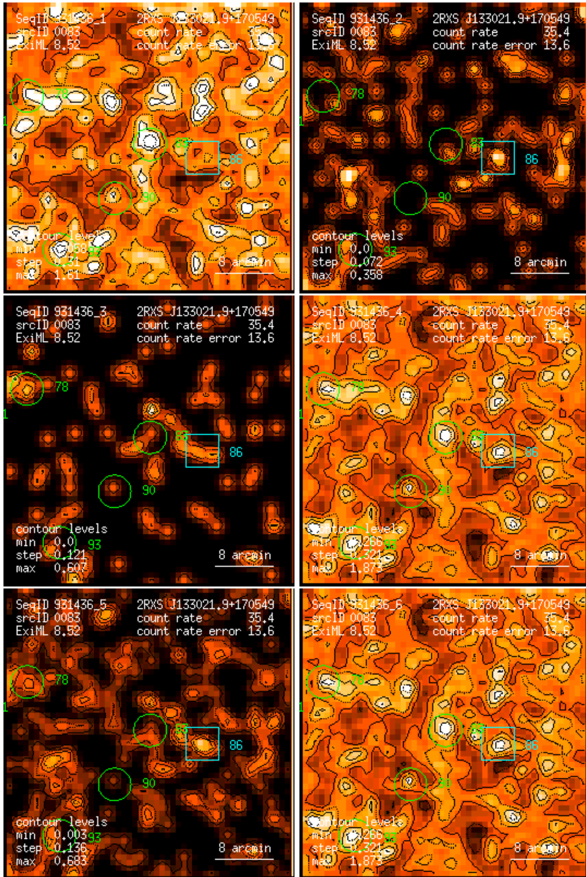
Figure 83: RASS 931436: detection 0083: band rate images, Gaussian filter: (1) PSPC channels 11 – 41, (2) 52 – 90, (3) 91 – 201, (4) 11 – 235, (5) 52 – 201, (6) 11 – 201. Broad band rates in counts/ks. Band rate contour levels in counts/ks/arcmin 2 .
