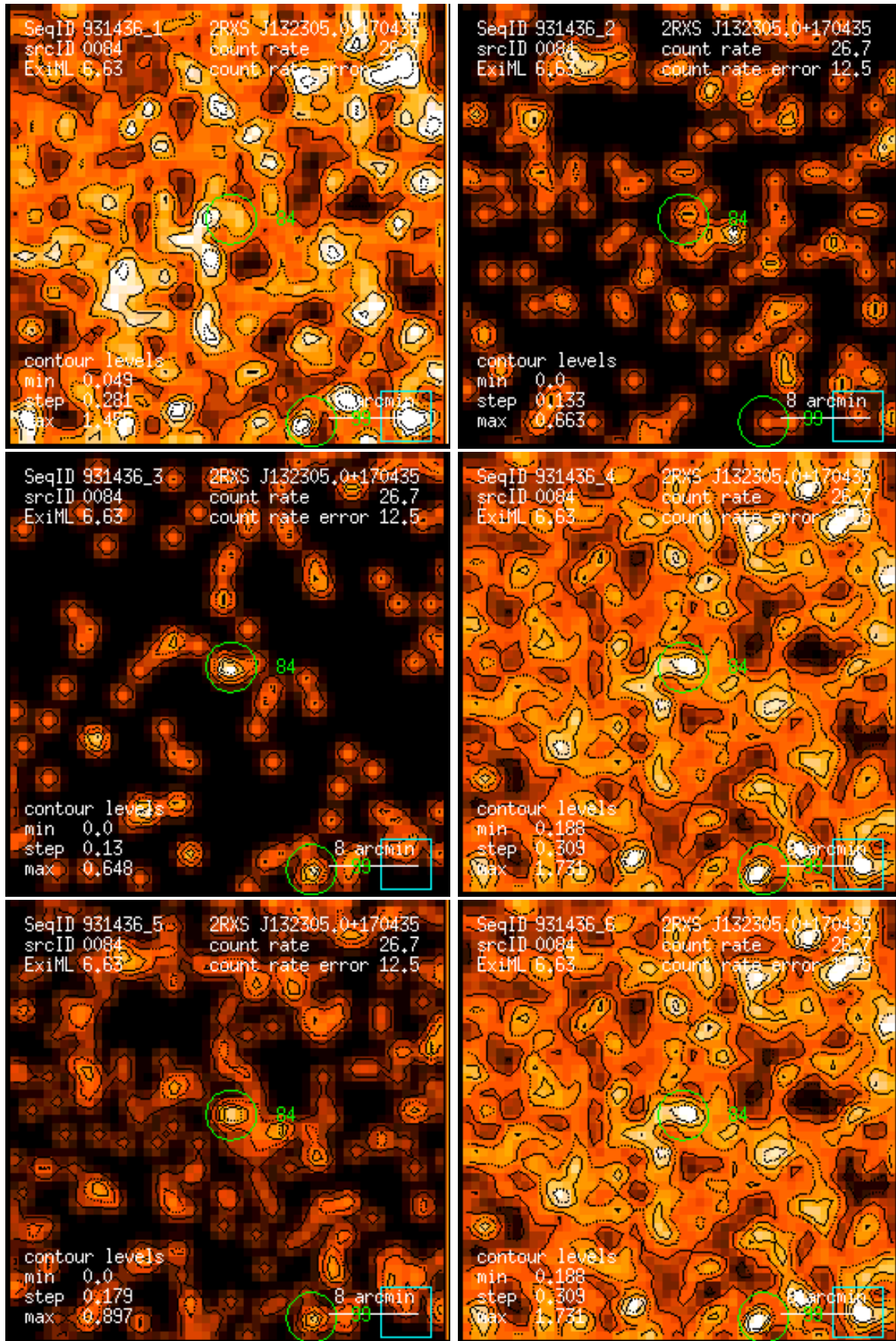
Figure 84: RASS 931436: detection 0084: band rate images, Gaussian filter: (1) PSPC channels 11 – 41, (2) 52 – 90, (3) 91 – 201, (4) 11 – 235, (5) 52 – 201, (6) 11 – 201. Broad band rates in counts/ks. Band rate contour levels in counts/ks/arcmin 2 .
