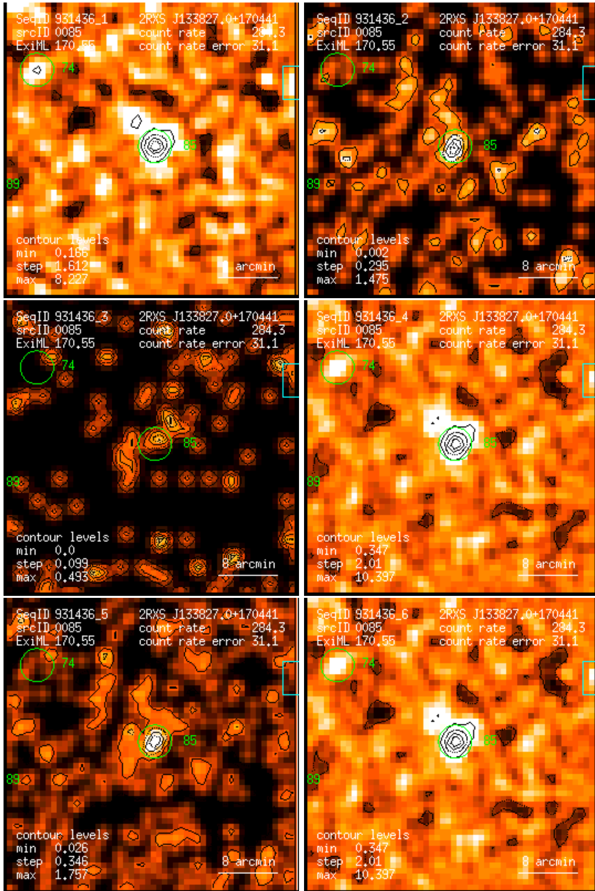
Figure 85: RASS 931436: detection 0085: band rate images, Gaussian filter: (1) PSPC channels 11 – 41, (2) 52 – 90, (3) 91 – 201, (4) 11 – 235, (5) 52 – 201, (6) 11 – 201. Broad band rates in counts/ks. Band rate contour levels in counts/ks/arcmin 2 .
