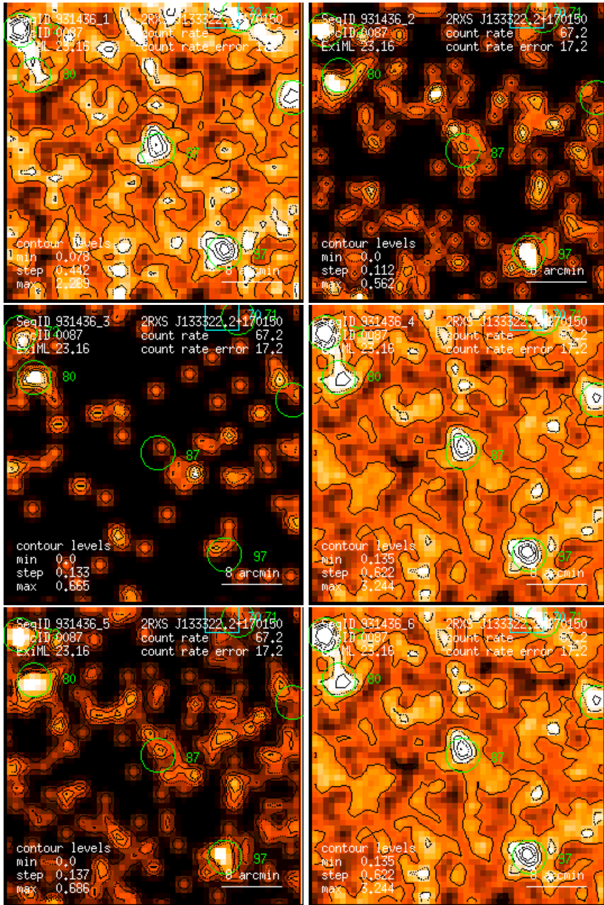
Figure 87: RASS 931436: detection 0087: band rate images, Gaussian filter: (1) PSPC channels 11 – 41, (2) 52 – 90, (3) 91 – 201, (4) 11 – 235, (5) 52 – 201, (6) 11 – 201. Broad band rates in counts/ks. Band rate contour levels in counts/ks/arcmin 2 .
