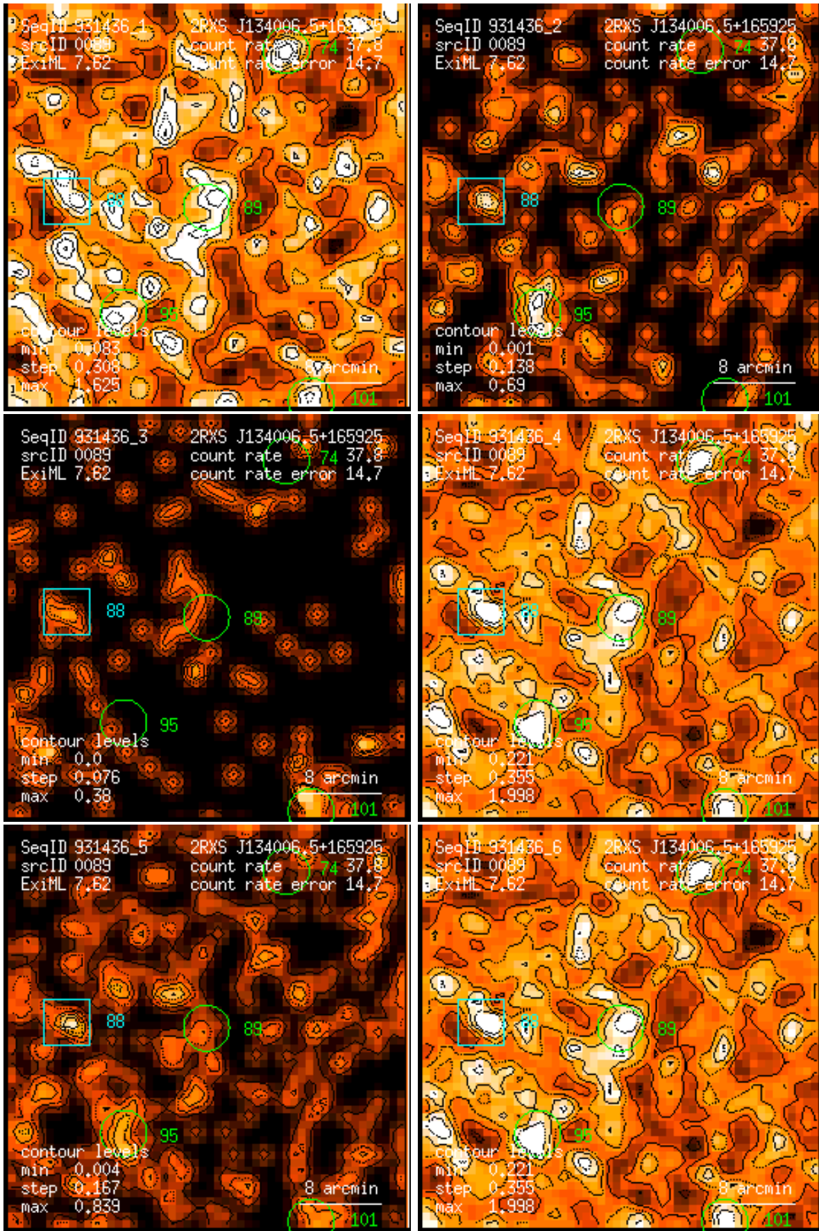
Figure 89: RASS 931436: detection 0089: band rate images, Gaussian filter: (1) PSPC channels 11 – 41, (2) 52 – 90, (3) 91 – 201, (4) 11 – 235, (5) 52 – 201, (6) 11 – 201. Broad band rates in counts/ks. Band rate contour levels in counts/ks/arcmin 2 .
