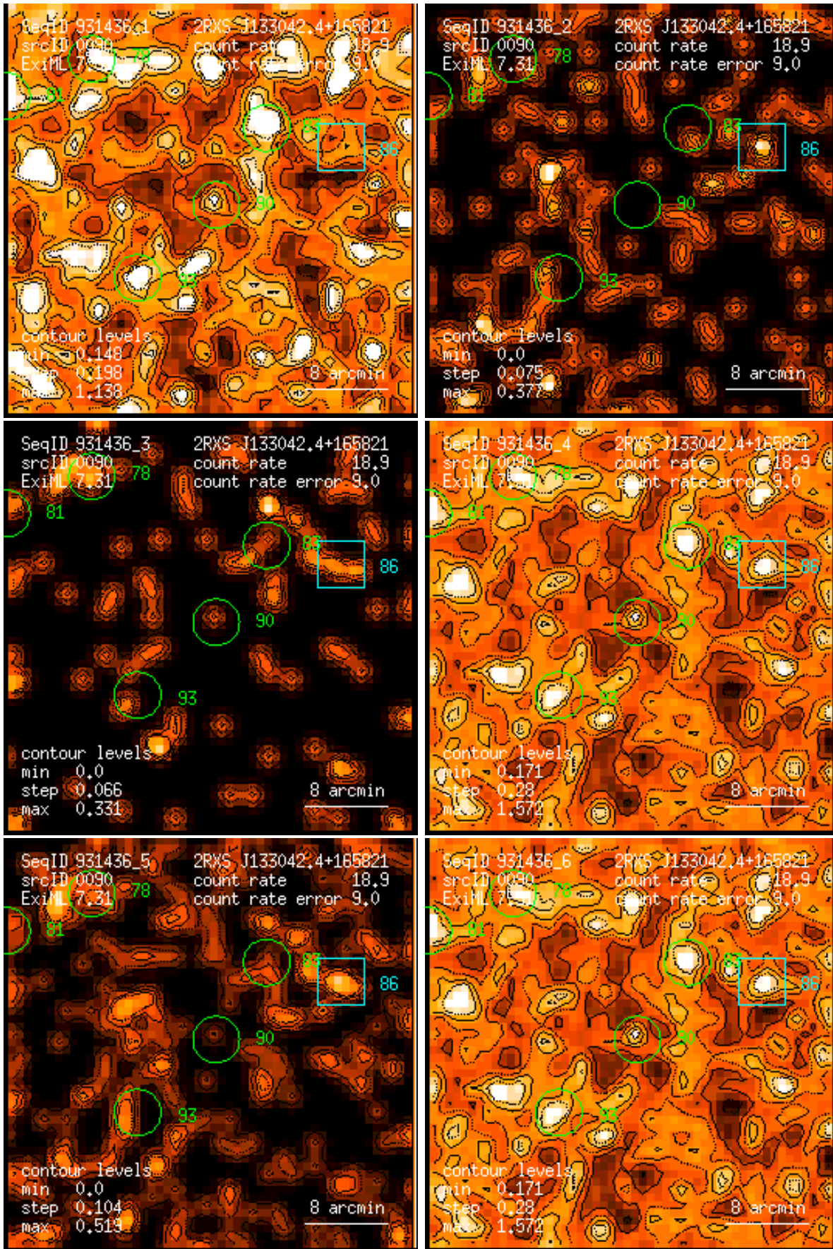
Figure 90: RASS 931436: detection 0090: band rate images, Gaussian filter: (1) PSPC channels 11 – 41, (2) 52 – 90, (3) 91 – 201, (4) 11 – 235, (5) 52 – 201, (6) 11 – 201. Broad band rates in counts/ks. Band rate contour levels in counts/ks/arcmin 2 .
