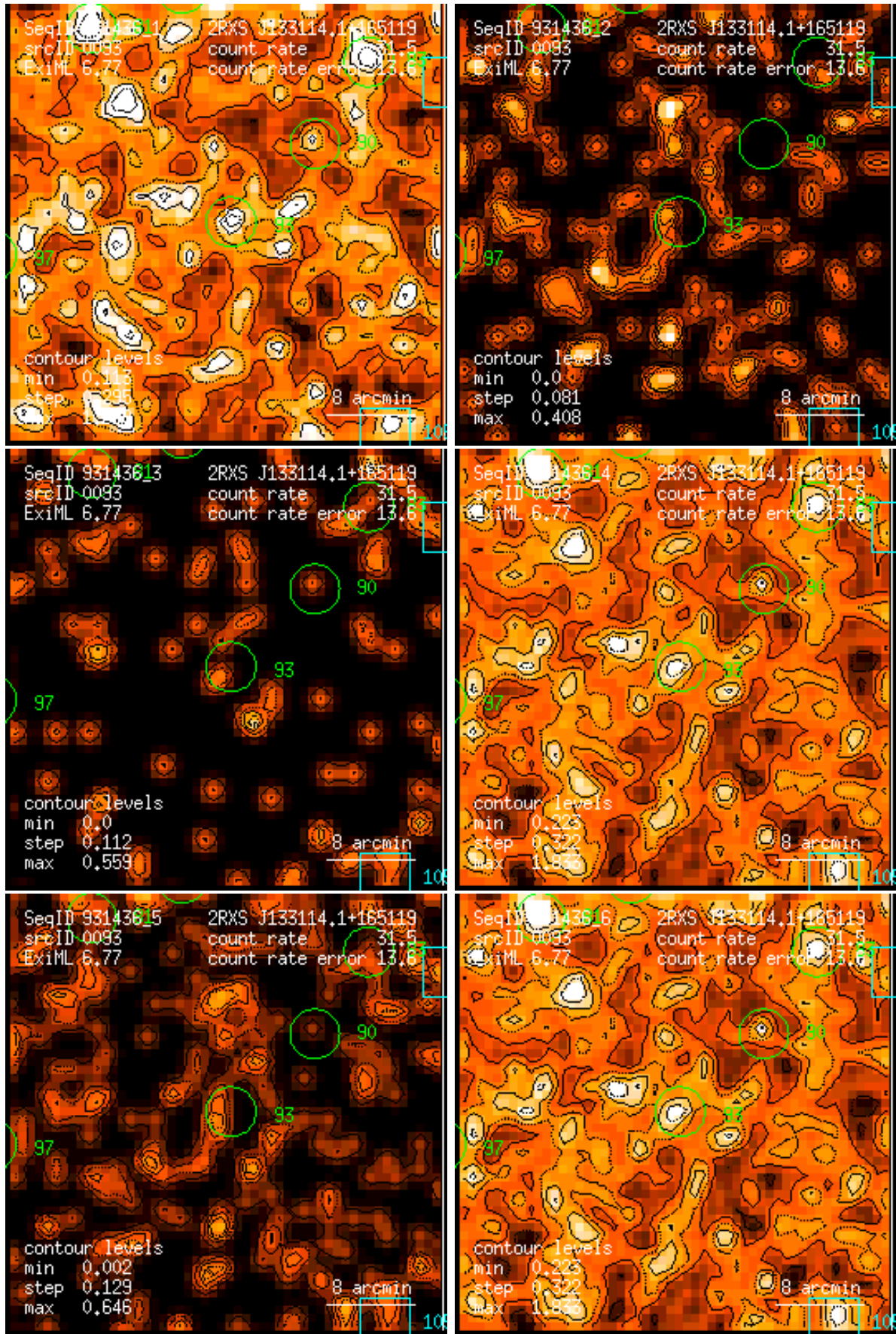
Figure 93: RASS 931436: detection 0093: band rate images, Gaussian filter: (1) PSPC channels 11 – 41, (2) 52 – 90, (3) 91 – 201, (4) 11 – 235, (5) 52 – 201, (6) 11 – 201. Broad band rates in counts/ks. Band rate contour levels in counts/ks/arcmin 2 .
