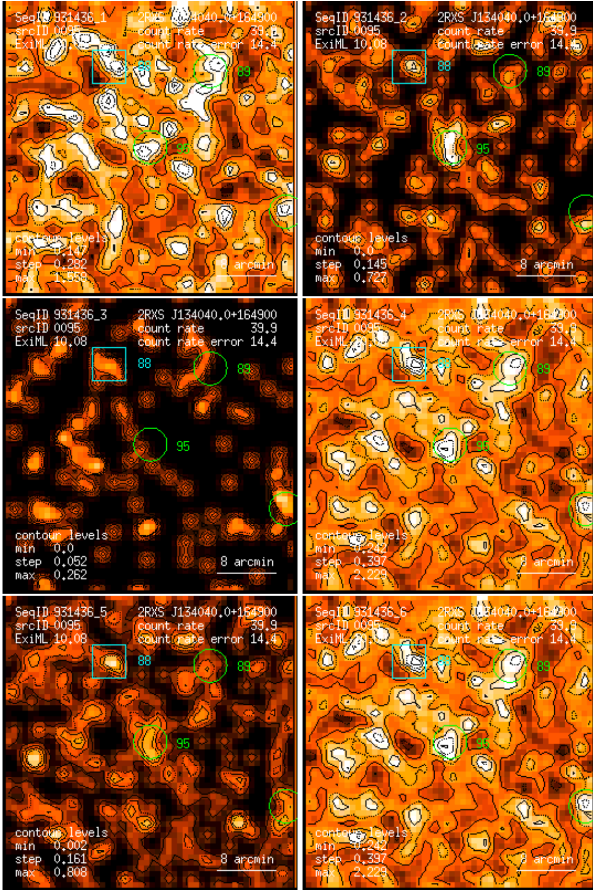
Figure 95: RASS 931436: detection 0095: band rate images, Gaussian filter: (1) PSPC channels 11 – 41, (2) 52 – 90, (3) 91 – 201, (4) 11 – 235, (5) 52 – 201, (6) 11 – 201. Broad band rates in counts/ks. Band rate contour levels in counts/ks/arcmin 2 .
