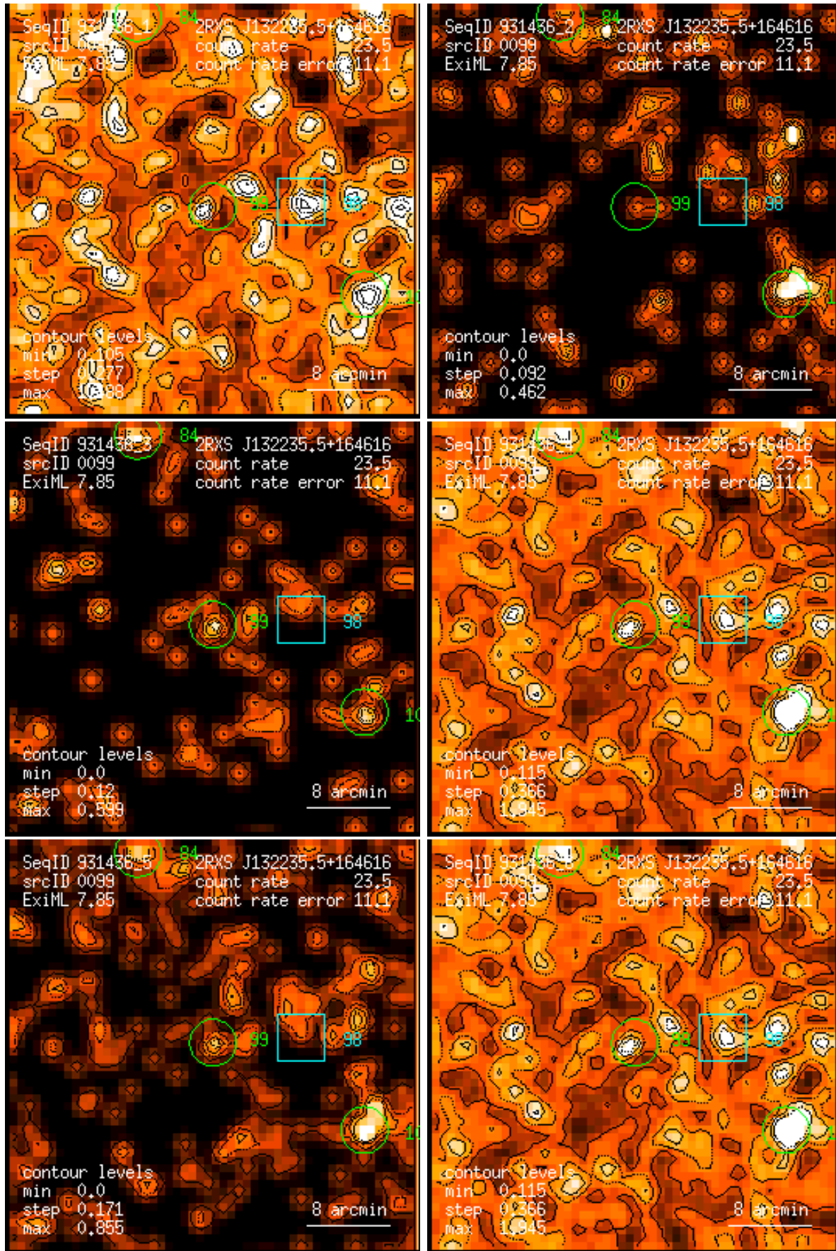
Figure 99: RASS 931436: detection 0099: band rate images, Gaussian filter: (1) PSPC channels 11 – 41, (2) 52 – 90, (3) 91 – 201, (4) 11 – 235, (5) 52 – 201, (6) 11 – 201. Broad band rates in counts/ks. Band rate contour levels in counts/ks/arcmin 2 .
