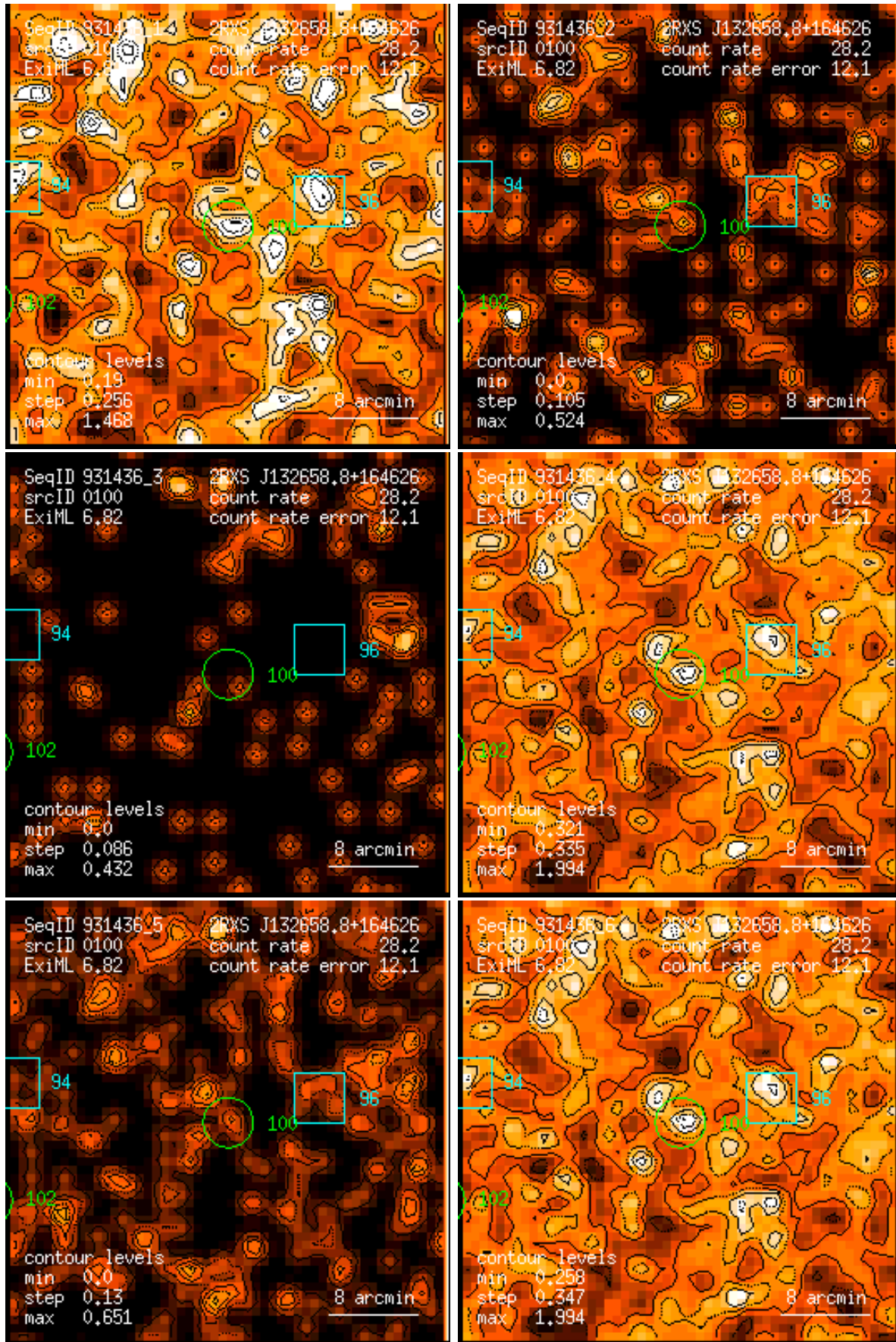
Figure 100: RASS 931436: detection 0100: band rate images, Gaussian filter: (1) PSPC channels 11 – 41, (2) 52 – 90, (3) 91 – 201, (4) 11 – 235, (5) 52 – 201, (6) 11 – 201. Broad band rates in counts/ks. Band rate contour levels in counts/ks/arcmin 2 .
