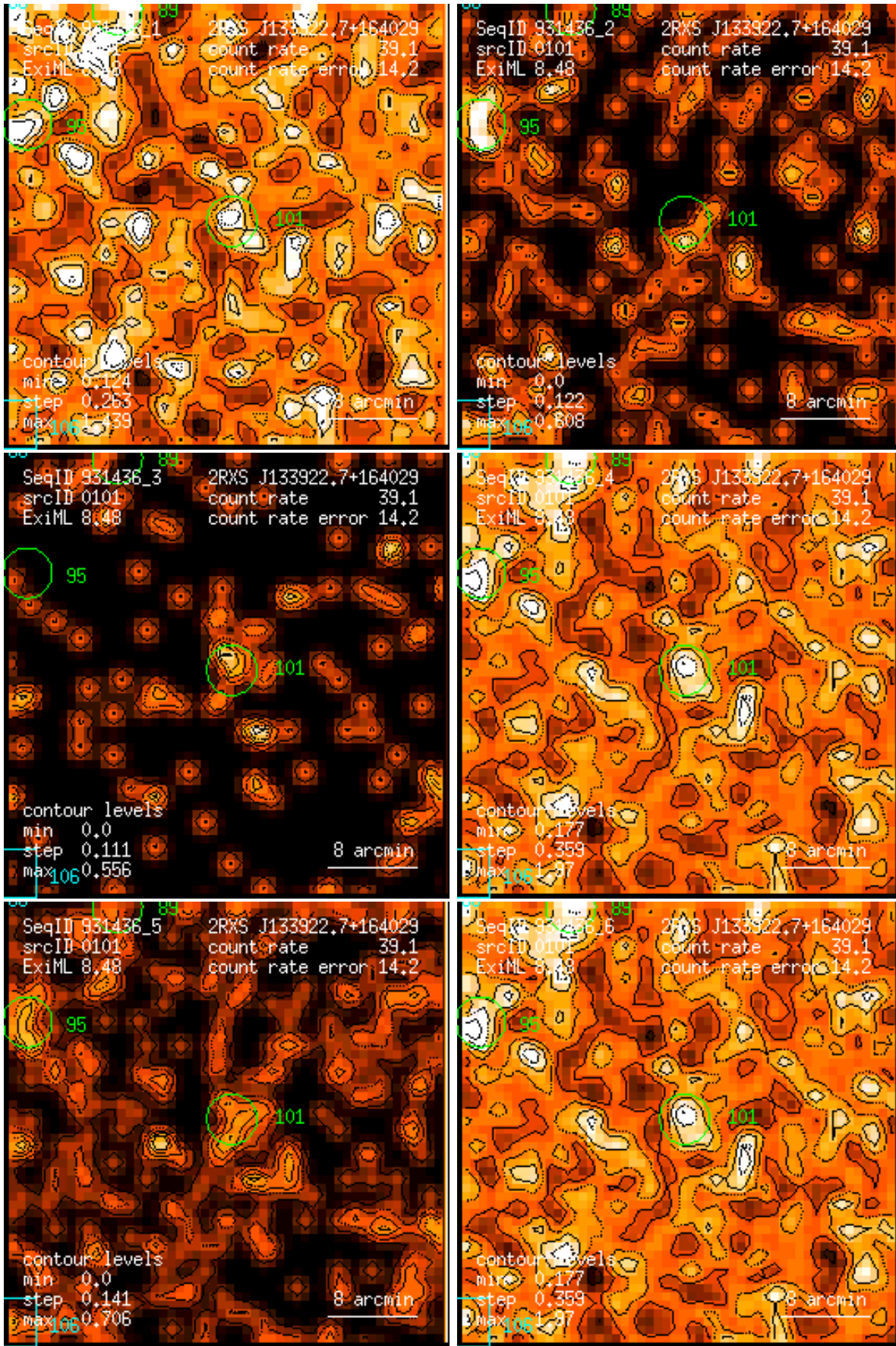
Figure 101: RASS 931436: detection 0101: band rate images, Gaussian filter: (1) PSPC channels 11 – 41, (2) 52 – 90, (3) 91 – 201, (4) 11 – 235, (5) 52 – 201, (6) 11 – 201. Broad band rates in counts/ks. Band rate contour levels in counts/ks/arcmin 2 .
