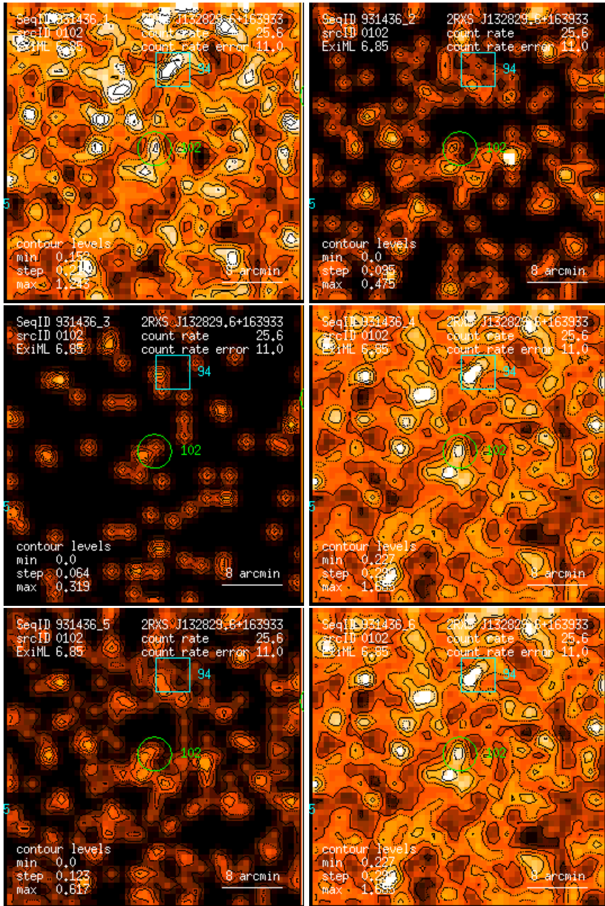
Figure 102: RASS 931436: detection 0102: band rate images, Gaussian filter: (1) PSPC channels 11 – 41, (2) 52 – 90, (3) 91 – 201, (4) 11 – 235, (5) 52 – 201, (6) 11 – 201. Broad band rates in counts/ks. Band rate contour levels in counts/ks/arcmin 2 .
