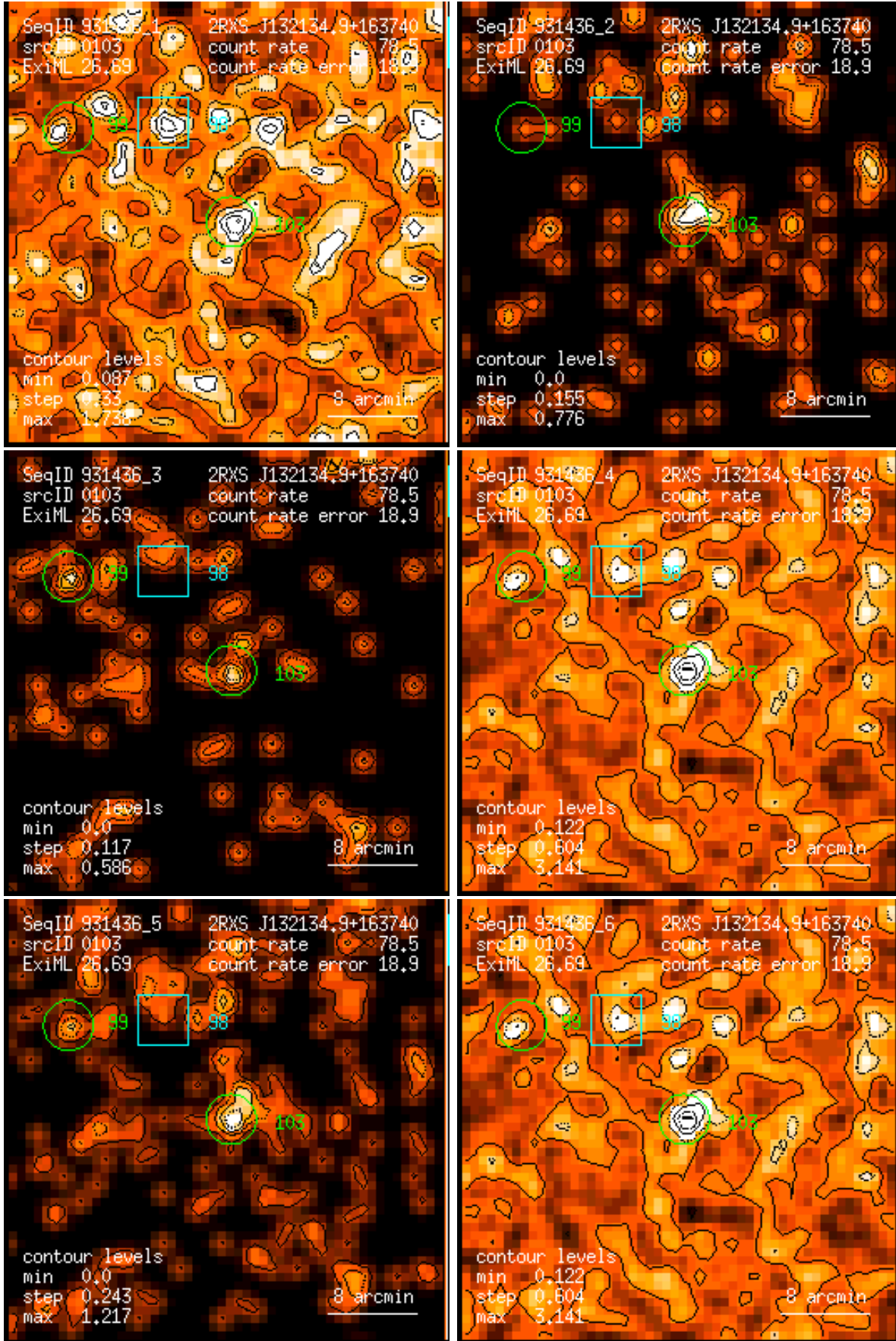
Figure 103: RASS 931436: detection 0103: band rate images, Gaussian filter: (1) PSPC channels 11 – 41, (2) 52 – 90, (3) 91 – 201, (4) 11 – 235, (5) 52 – 201, (6) 11 – 201. Broad band rates in counts/ks. Band rate contour levels in counts/ks/arcmin 2 .
