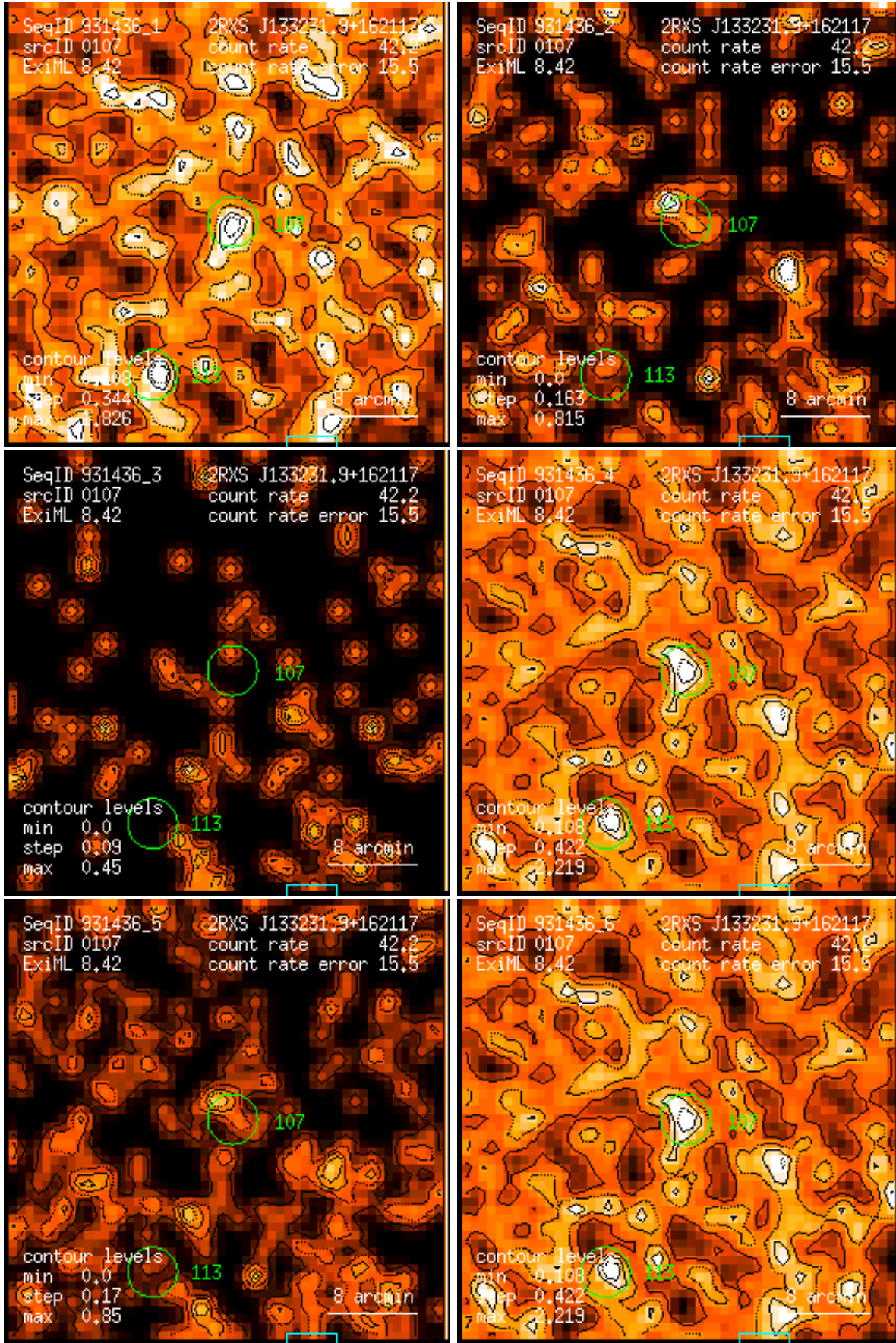
Figure 107: RASS 931436: detection 0107: band rate images, Gaussian filter: (1) PSPC channels 11 – 41, (2) 52 – 90, (3) 91 – 201, (4) 11 – 235, (5) 52 – 201, (6) 11 – 201. Broad band rates in counts/ks. Band rate contour levels in counts/ks/arcmin 2 .
