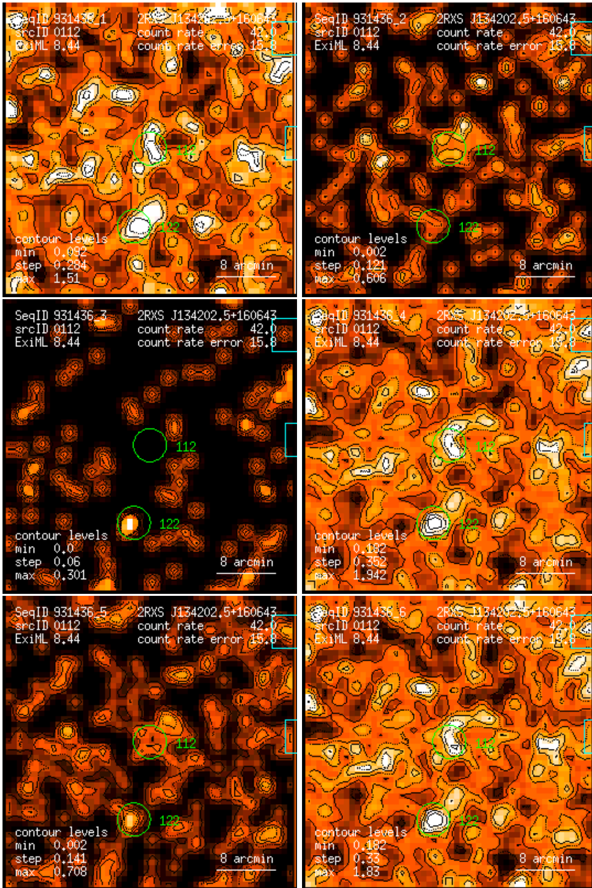
Figure 112: RASS 931436: detection 0112: band rate images, Gaussian filter: (1) PSPC channels 11 – 41, (2) 52 – 90, (3) 91 – 201, (4) 11 – 235, (5) 52 – 201, (6) 11 – 201. Broad band rates in counts/ks. Band rate contour levels in counts/ks/arcmin 2 .
