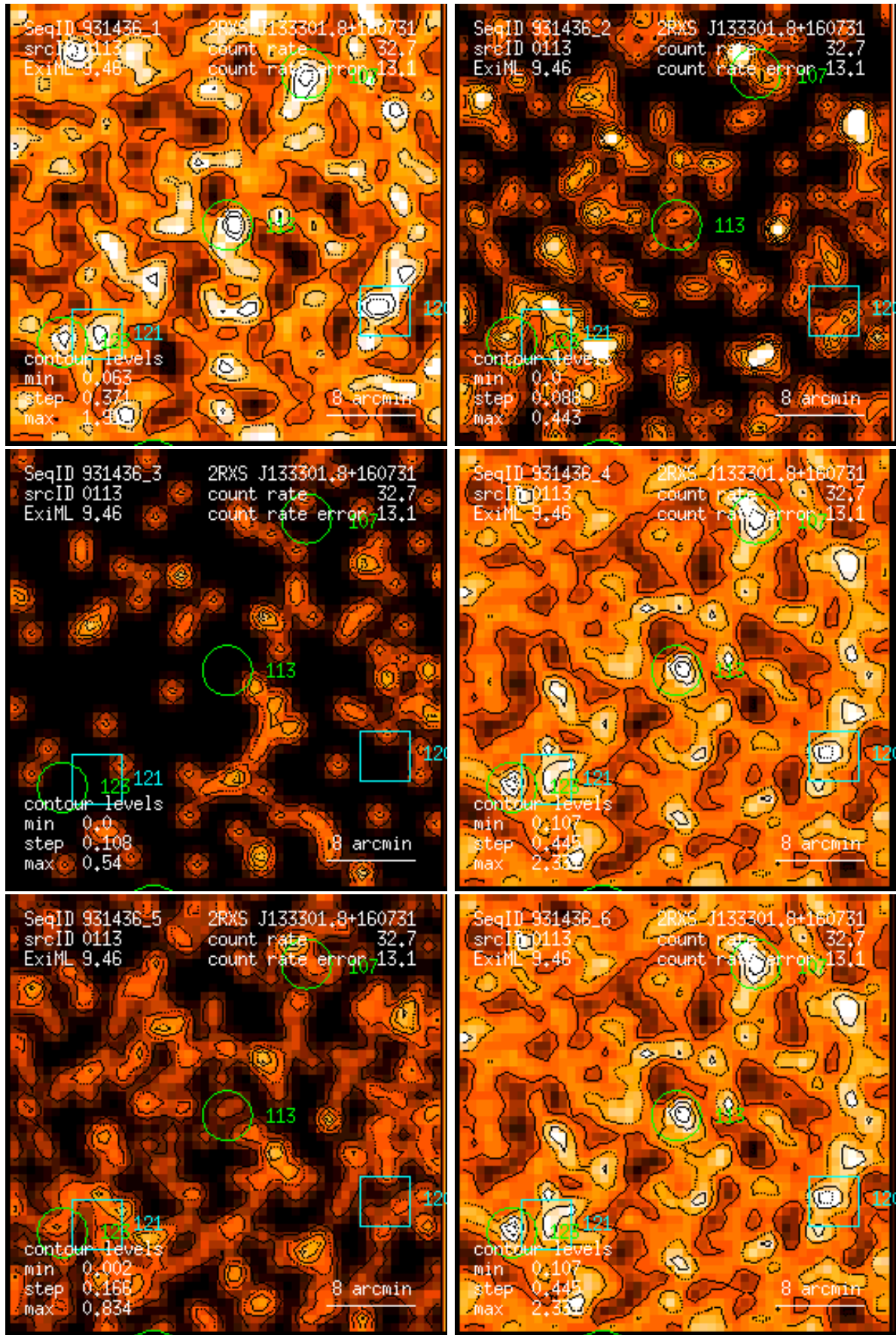
Figure 113: RASS 931436: detection 0113: band rate images, Gaussian filter: (1) PSPC channels 11 – 41, (2) 52 – 90, (3) 91 – 201, (4) 11 – 235, (5) 52 – 201, (6) 11 – 201. Broad band rates in counts/ks. Band rate contour levels in counts/ks/arcmin 2 .
