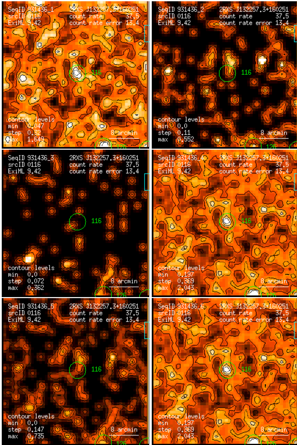
Figure 116: RASS 931436: detection 0116: band rate images, Gaussian filter: (1) PSPC channels 11 – 41, (2) 52 – 90, (3) 91 – 201, (4) 11 – 235, (5) 52 – 201, (6) 11 – 201. Broad band rates in counts/ks. Band rate contour levels in counts/ks/arcmin 2 .
