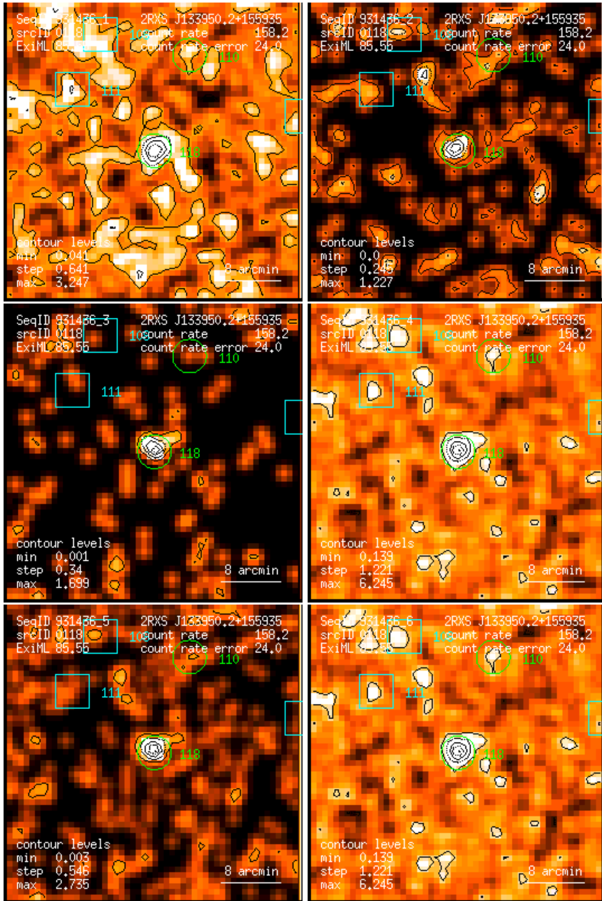
Figure 118: RASS 931436: detection 0118: band rate images, Gaussian filter: (1) PSPC channels 11 – 41, (2) 52 – 90, (3) 91 – 201, (4) 11 – 235, (5) 52 – 201, (6) 11 – 201. Broad band rates in counts/ks. Band rate contour levels in counts/ks/arcmin 2 .
