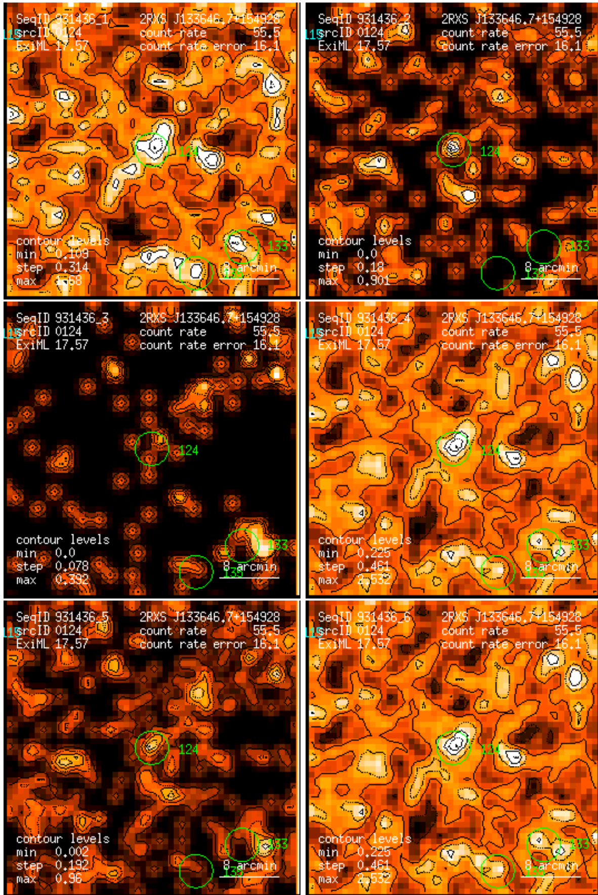
Figure 124: RASS 931436: detection 0124: band rate images, Gaussian filter: (1) PSPC channels 11 – 41, (2) 52 – 90, (3) 91 – 201, (4) 11 – 235, (5) 52 – 201, (6) 11 – 201. Broad band rates in counts/ks. Band rate contour levels in counts/ks/arcmin 2 .
