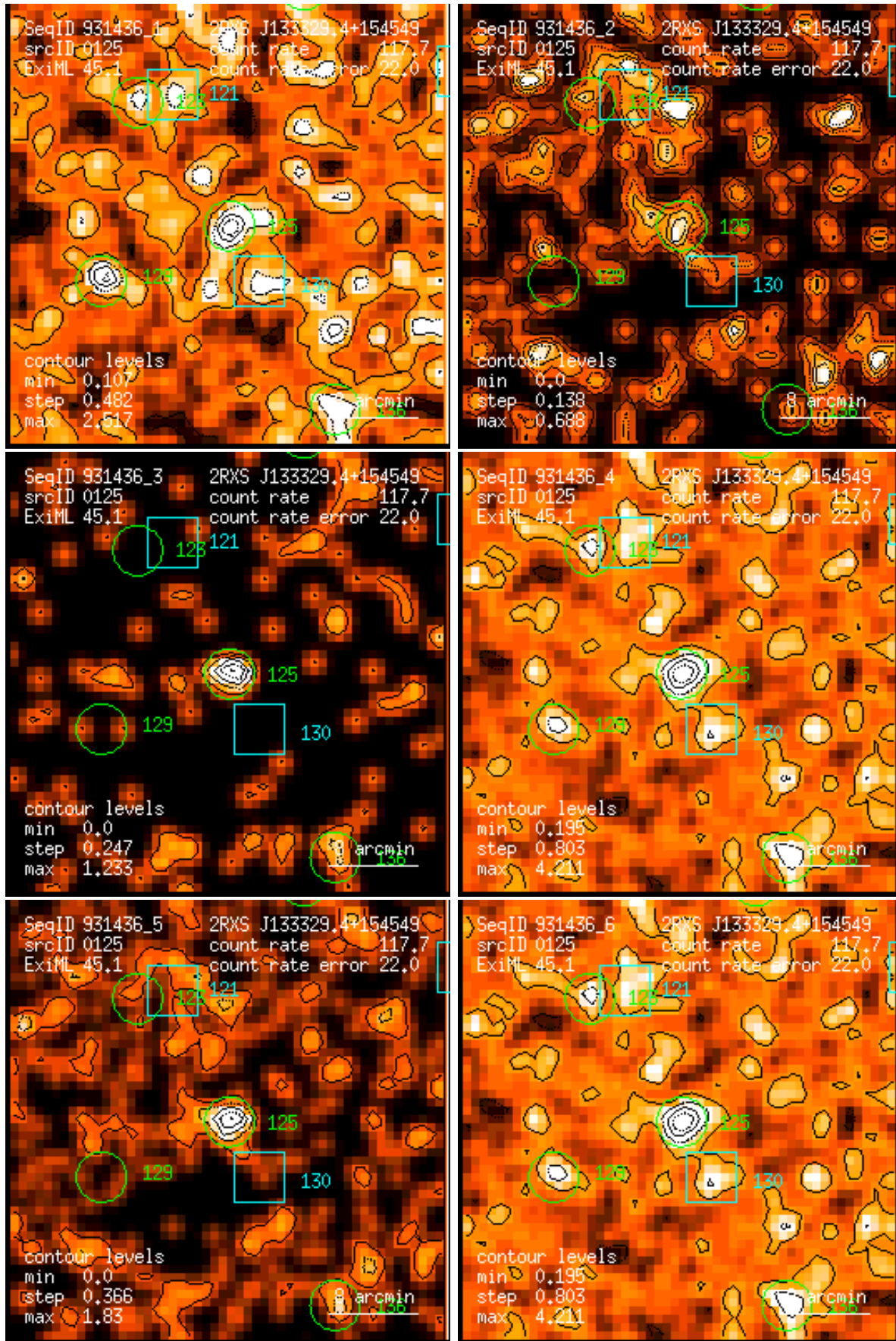
Figure 125: RASS 931436: detection 0125: band rate images, Gaussian filter: (1) PSPC channels 11 – 41, (2) 52 – 90, (3) 91 – 201, (4) 11 – 235, (5) 52 – 201, (6) 11 – 201. Broad band rates in counts/ks. Band rate contour levels in counts/ks/arcmin 2 .
