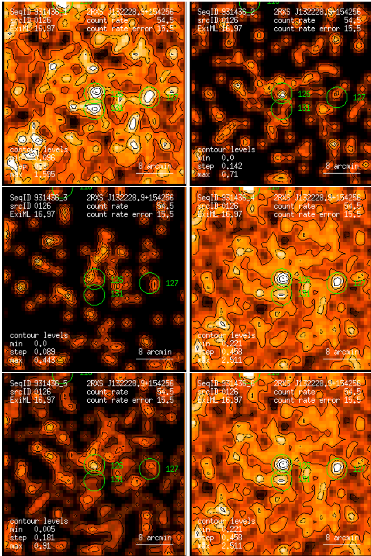
Figure 126: RASS 931436: detection 0126: band rate images, Gaussian filter: (1) PSPC channels 11 – 41, (2) 52 – 90, (3) 91 – 201, (4) 11 – 235, (5) 52 – 201, (6) 11 – 201. Broad band rates in counts/ks. Band rate contour levels in counts/ks/arcmin 2 .
