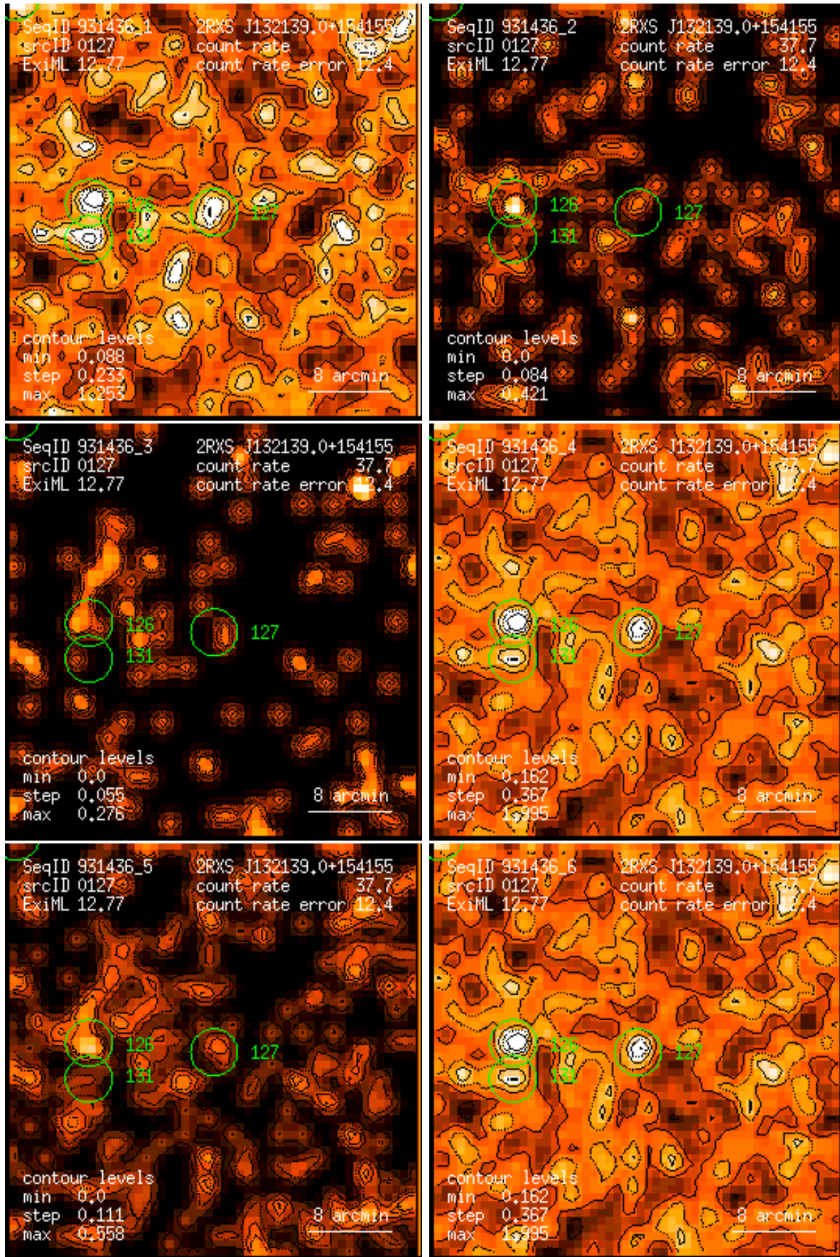
Figure 127: RASS 931436: detection 0127: band rate images, Gaussian filter: (1) PSPC channels 11 – 41, (2) 52 – 90, (3) 91 – 201, (4) 11 – 235, (5) 52 – 201, (6) 11 – 201. Broad band rates in counts/ks. Band rate contour levels in counts/ks/arcmin 2 .
