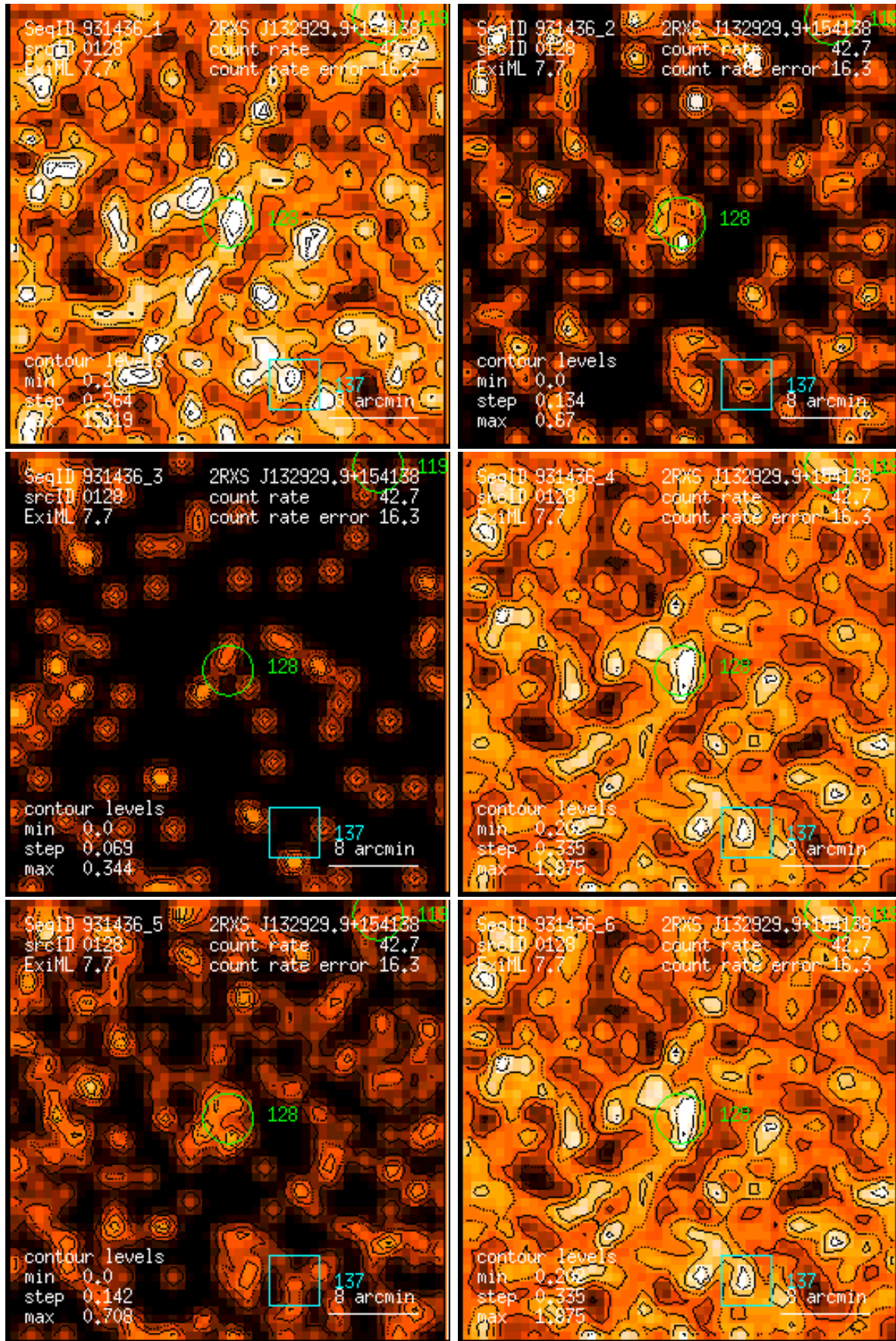
Figure 128: RASS 931436: detection 0128: band rate images, Gaussian filter: (1) PSPC channels 11 – 41, (2) 52 – 90, (3) 91 – 201, (4) 11 – 235, (5) 52 – 201, (6) 11 – 201. Broad band rates in counts/ks. Band rate contour levels in counts/ks/arcmin 2 .
