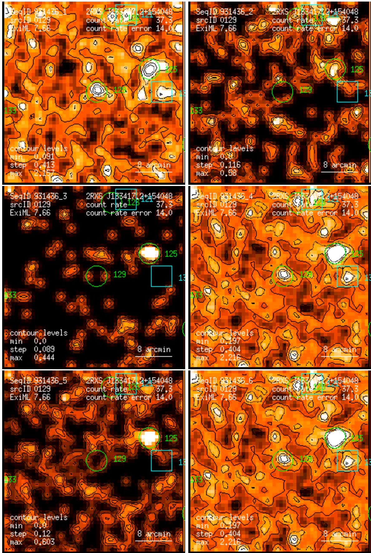
Figure 129: RASS 931436: detection 0129: band rate images, Gaussian filter: (1) PSPC channels 11 – 41, (2) 52 – 90, (3) 91 – 201, (4) 11 – 235, (5) 52 – 201, (6) 11 – 201. Broad band rates in counts/ks. Band rate contour levels in counts/ks/arcmin 2 .
