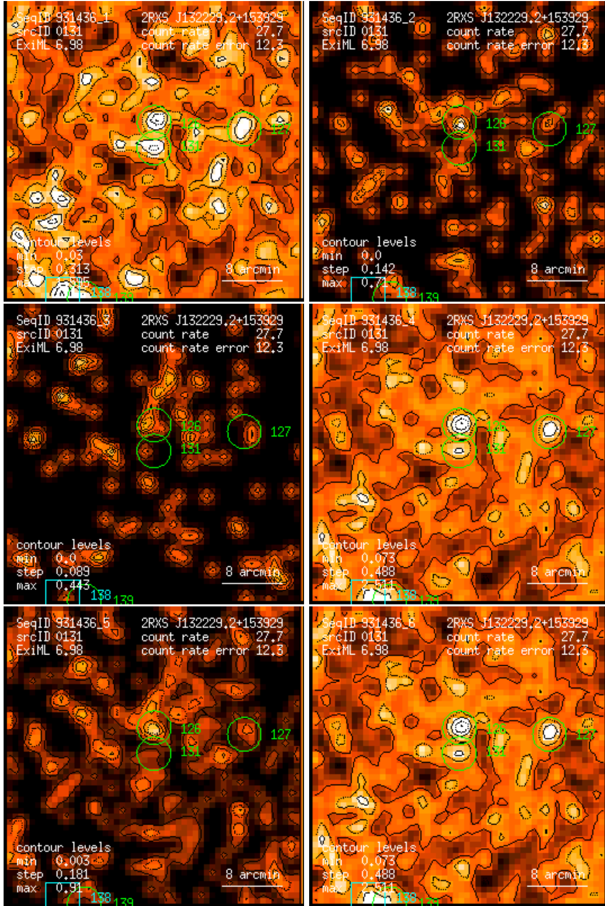
Figure 131: RASS 931436: detection 0131: band rate images, Gaussian filter: (1) PSPC channels 11 – 41, (2) 52 – 90, (3) 91 – 201, (4) 11 – 235, (5) 52 – 201, (6) 11 – 201. Broad band rates in counts/ks. Band rate contour levels in counts/ks/arcmin 2 .
