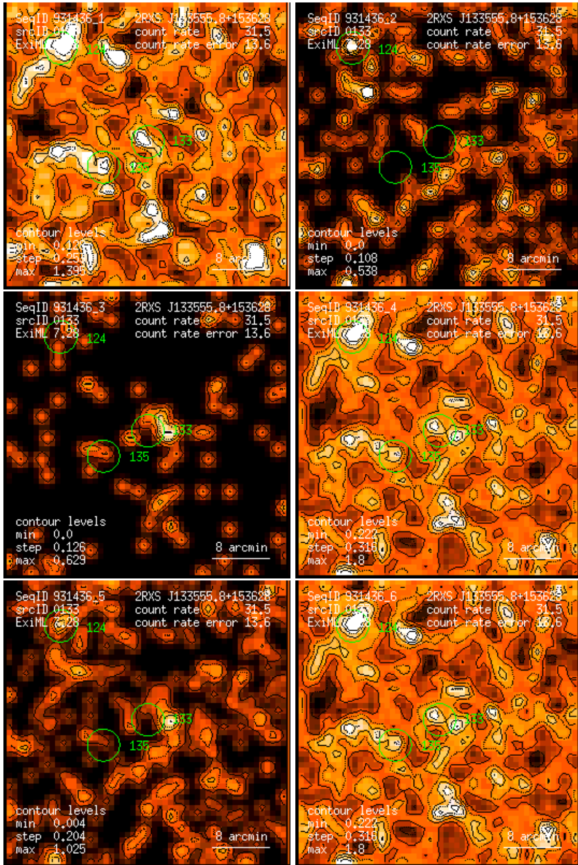
Figure 133: RASS 931436: detection 0133: band rate images, Gaussian filter: (1) PSPC channels 11 – 41, (2) 52 – 90, (3) 91 – 201, (4) 11 – 235, (5) 52 – 201, (6) 11 – 201. Broad band rates in counts/ks. Band rate contour levels in counts/ks/arcmin 2 .
