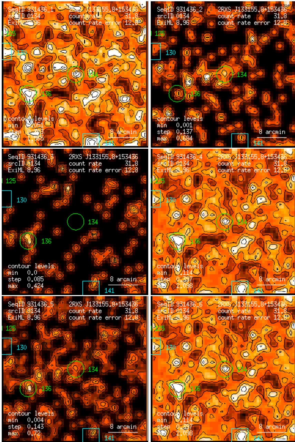
Figure 134: RASS 931436: detection 0134: band rate images, Gaussian filter: (1) PSPC channels 11 – 41, (2) 52 – 90, (3) 91 – 201, (4) 11 – 235, (5) 52 – 201, (6) 11 – 201. Broad band rates in counts/ks. Band rate contour levels in counts/ks/arcmin 2 .
