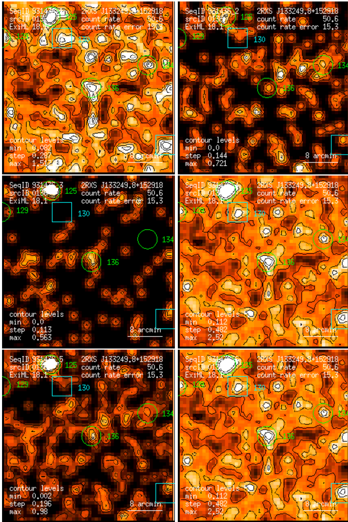
Figure 136: RASS 931436: detection 0136: band rate images, Gaussian filter: (1) PSPC channels 11 – 41, (2) 52 – 90, (3) 91 – 201, (4) 11 – 235, (5) 52 – 201, (6) 11 – 201. Broad band rates in counts/ks. Band rate contour levels in counts/ks/arcmin 2 .
