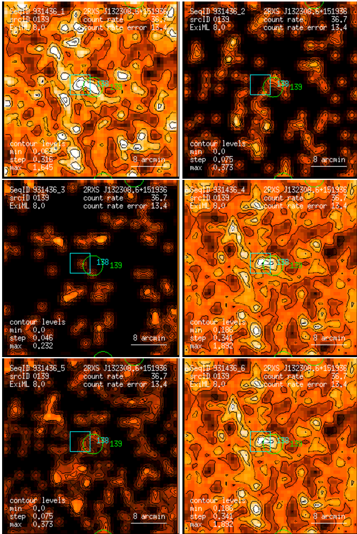
Figure 139: RASS 931436: detection 0139: band rate images, Gaussian filter: (1) PSPC channels 11 – 41, (2) 52 – 90, (3) 91 – 201, (4) 11 – 235, (5) 52 – 201, (6) 11 – 201. Broad band rates in counts/ks. Band rate contour levels in counts/ks/arcmin 2 .
