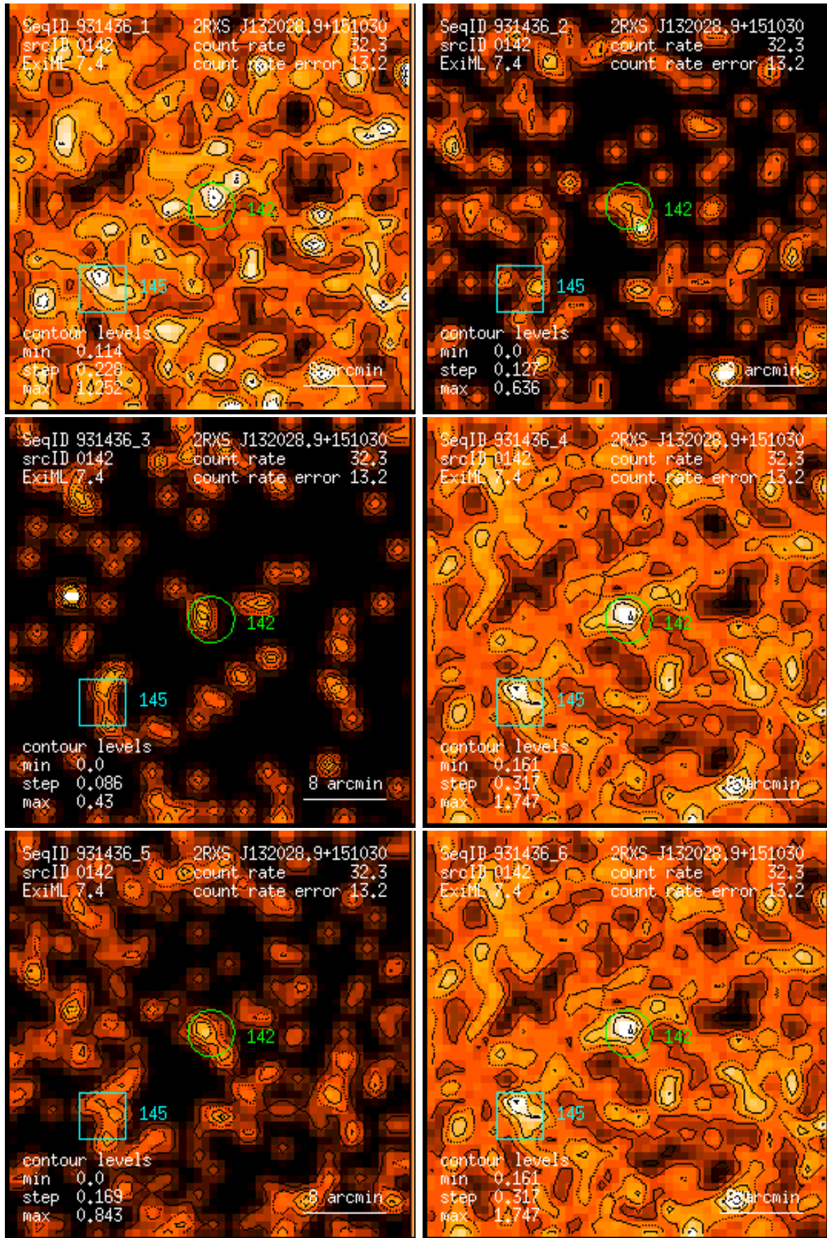
Figure 142: RASS 931436: detection 0142: band rate images, Gaussian filter: (1) PSPC channels 11 – 41, (2) 52 – 90, (3) 91 – 201, (4) 11 – 235, (5) 52 – 201, (6) 11 – 201. Broad band rates in counts/ks. Band rate contour levels in counts/ks/arcmin 2 .
