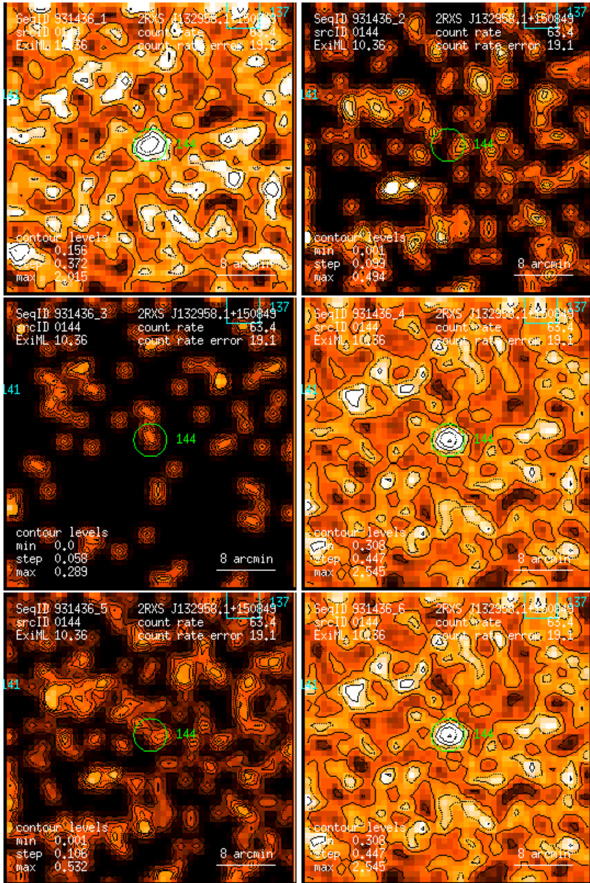
Figure 144: RASS 931436: detection 0144: band rate images, Gaussian filter: (1) PSPC channels 11 – 41, (2) 52 – 90, (3) 91 – 201, (4) 11 – 235, (5) 52 – 201, (6) 11 – 201. Broad band rates in counts/ks. Band rate contour levels in counts/ks/arcmin 2 .
