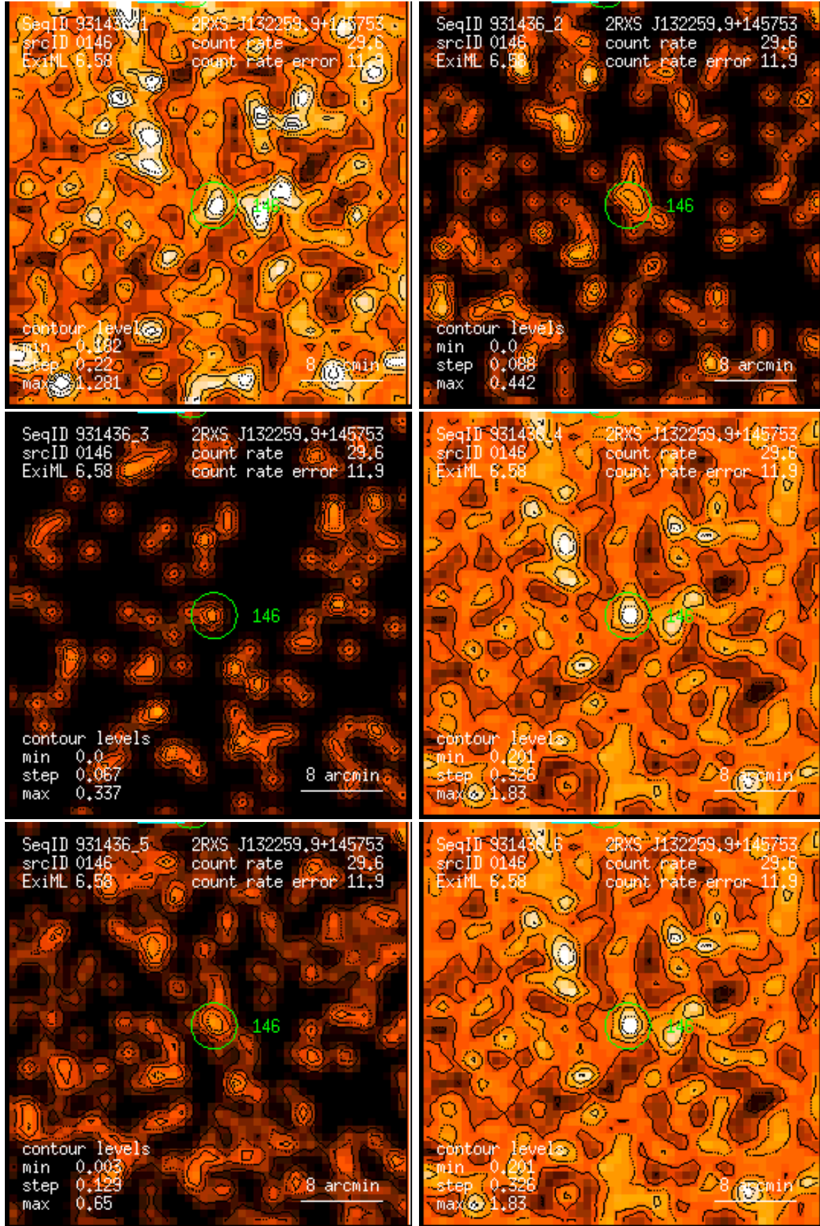
Figure 146: RASS 931436: detection 0146: band rate images, Gaussian filter: (1) PSPC channels 11 – 41, (2) 52 – 90, (3) 91 – 201, (4) 11 – 235, (5) 52 – 201, (6) 11 – 201. Broad band rates in counts/ks. Band rate contour levels in counts/ks/arcmin 2 .
