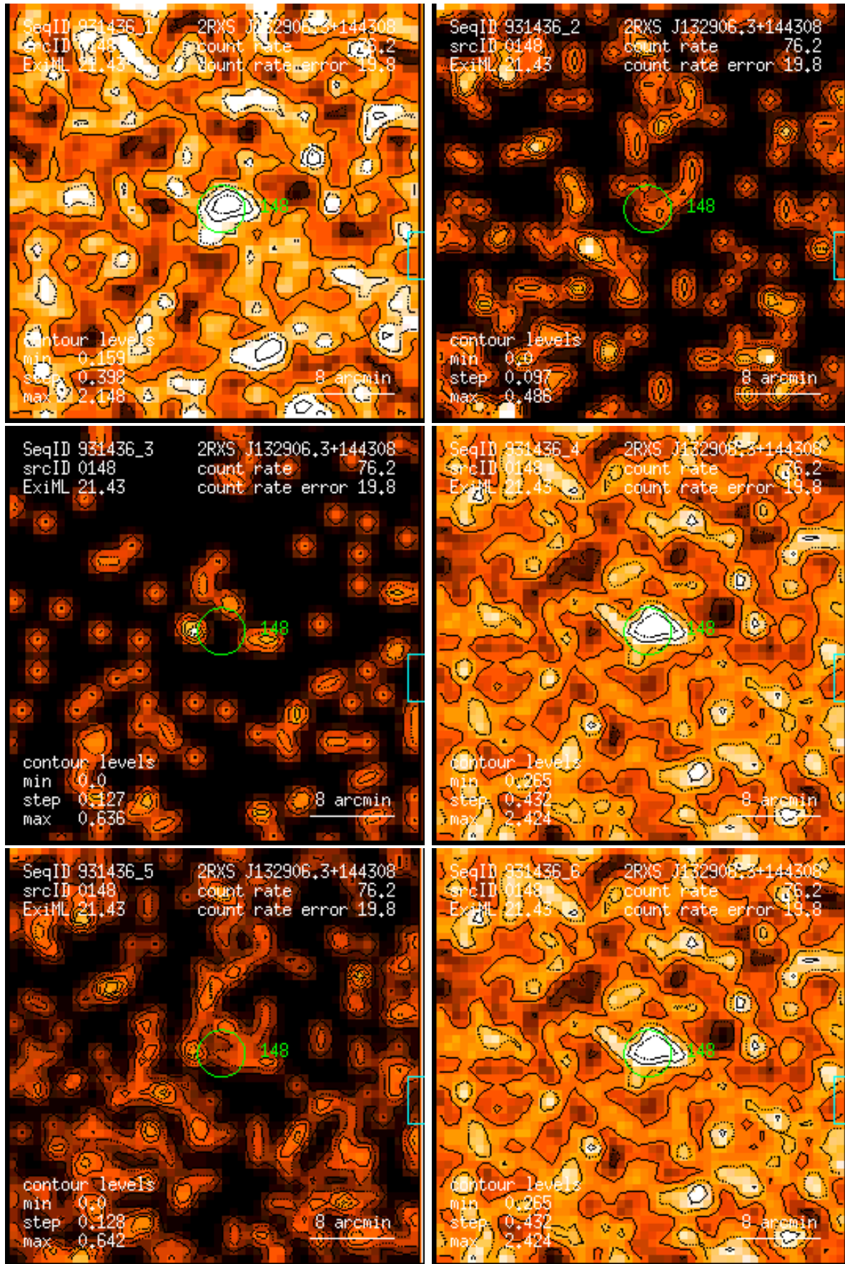
Figure 148: RASS 931436: detection 0148: band rate images, Gaussian filter: (1) PSPC channels 11 – 41, (2) 52 – 90, (3) 91 – 201, (4) 11 – 235, (5) 52 – 201, (6) 11 – 201. Broad band rates in counts/ks. Band rate contour levels in counts/ks/arcmin 2 .
