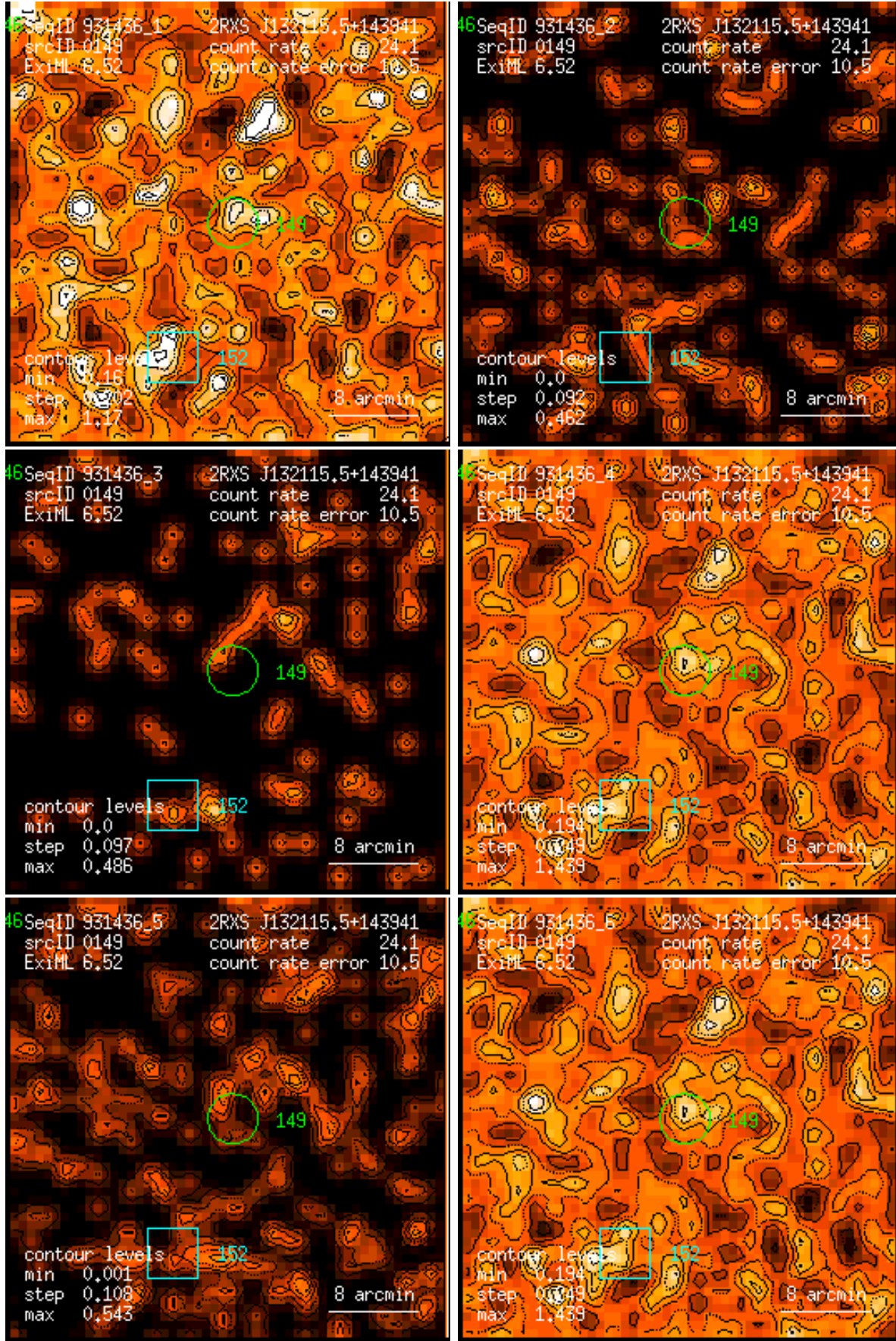
Figure 149: RASS 931436: detection 0149: band rate images, Gaussian filter: (1) PSPC channels 11 – 41, (2) 52 – 90, (3) 91 – 201, (4) 11 – 235, (5) 52 – 201, (6) 11 – 201. Broad band rates in counts/ks. Band rate contour levels in counts/ks/arcmin 2 .
