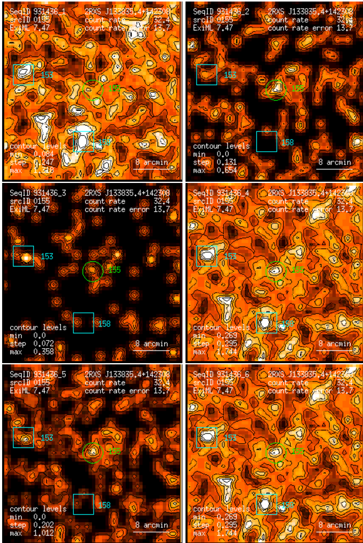
Figure 155: RASS 931436: detection 0155: band rate images, Gaussian filter: (1) PSPC channels 11 – 41, (2) 52 – 90, (3) 91 – 201, (4) 11 – 235, (5) 52 – 201, (6) 11 – 201. Broad band rates in counts/ks. Band rate contour levels in counts/ks/arcmin 2 .
