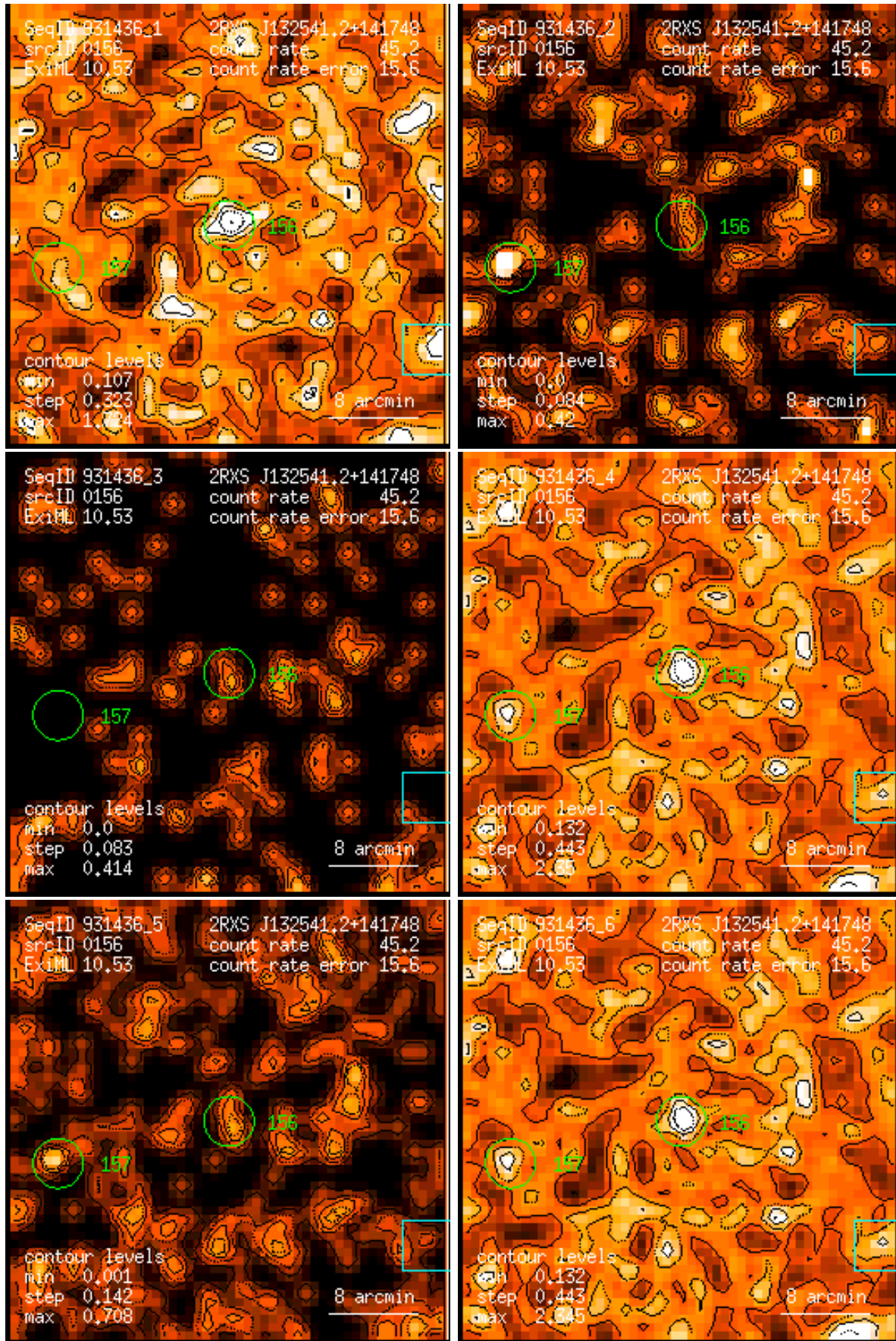
Figure 156: RASS 931436: detection 0156: band rate images, Gaussian filter: (1) PSPC channels 11 – 41, (2) 52 – 90, (3) 91 – 201, (4) 11 – 235, (5) 52 – 201, (6) 11 – 201. Broad band rates in counts/ks. Band rate contour levels in counts/ks/arcmin 2 .
