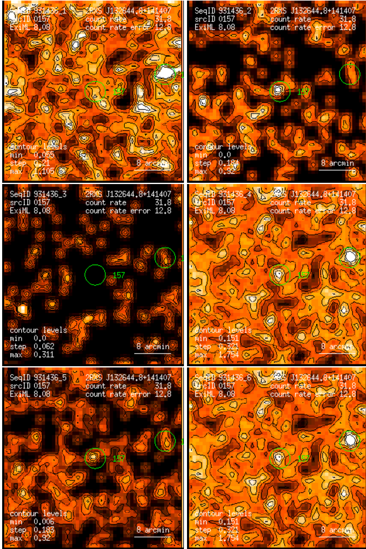
Figure 157: RASS 931436: detection 0157: band rate images, Gaussian filter: (1) PSPC channels 11 – 41, (2) 52 – 90, (3) 91 – 201, (4) 11 – 235, (5) 52 – 201, (6) 11 – 201. Broad band rates in counts/ks. Band rate contour levels in counts/ks/arcmin 2 .
