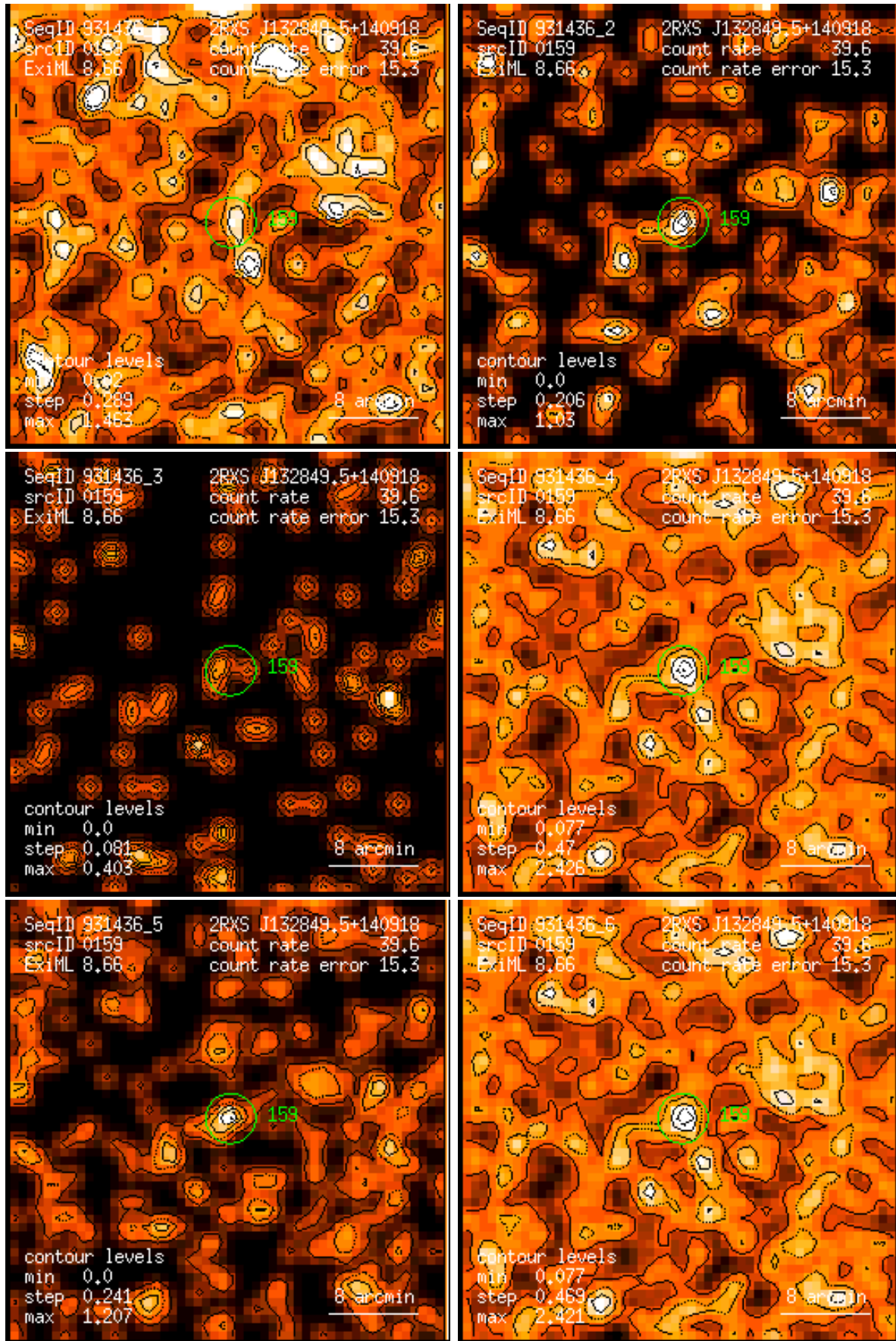
Figure 159: RASS 931436: detection 0159: band rate images, Gaussian filter: (1) PSPC channels 11 – 41, (2) 52 – 90, (3) 91 – 201, (4) 11 – 235, (5) 52 – 201, (6) 11 – 201. Broad band rates in counts/ks. Band rate contour levels in counts/ks/arcmin 2 .
