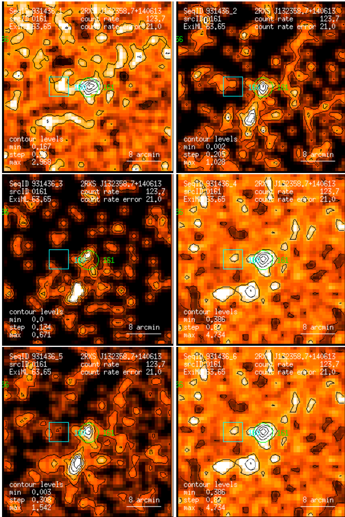
Figure 161: RASS 931436: detection 0161: band rate images, Gaussian filter: (1) PSPC channels 11 – 41, (2) 52 – 90, (3) 91 – 201, (4) 11 – 235, (5) 52 – 201, (6) 11 – 201. Broad band rates in counts/ks. Band rate contour levels in counts/ks/arcmin 2 .
