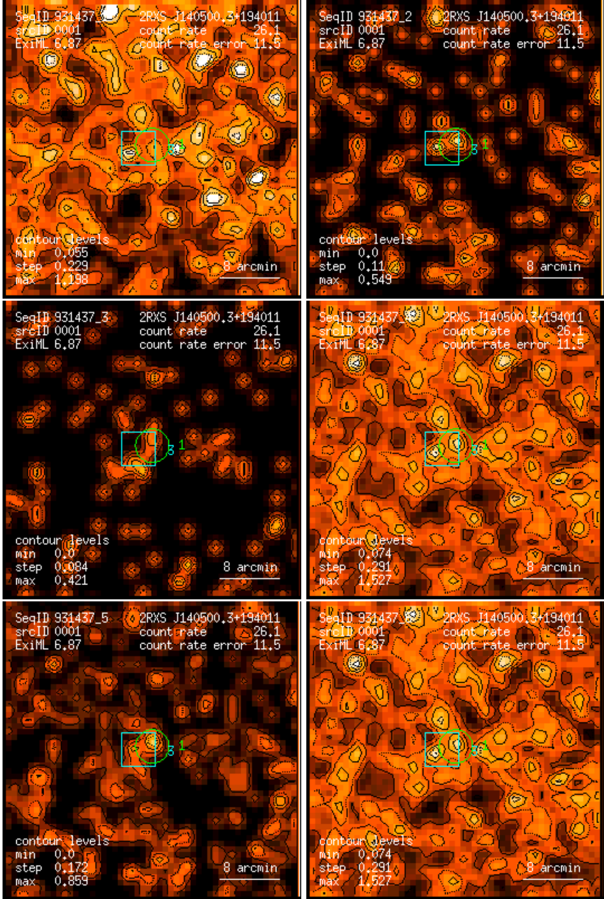
Figure 1: RASS 931437: detection 0001: band rate images, Gaussian filter: (1) PSPC channels 11 – 41, (2) 52 – 90, (3) 91 – 201, (4) 11 – 235, (5) 52 – 201, (6) 11 – 201. Broad band rates in counts/ks. Band rate contour levels in counts/ks/arcmin 2 .
