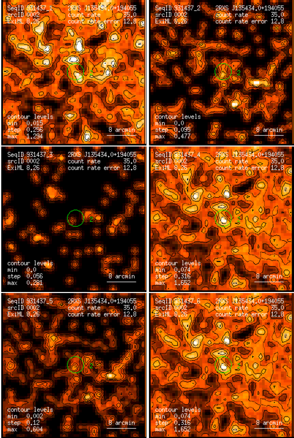
Figure 2: RASS 931437: detection 0002: band rate images, Gaussian filter: (1) PSPC channels 11 – 41, (2) 52 – 90, (3) 91 – 201, (4) 11 – 235, (5) 52 – 201, (6) 11 – 201. Broad band rates in counts/ks. Band rate contour levels in counts/ks/arcmin 2 .
