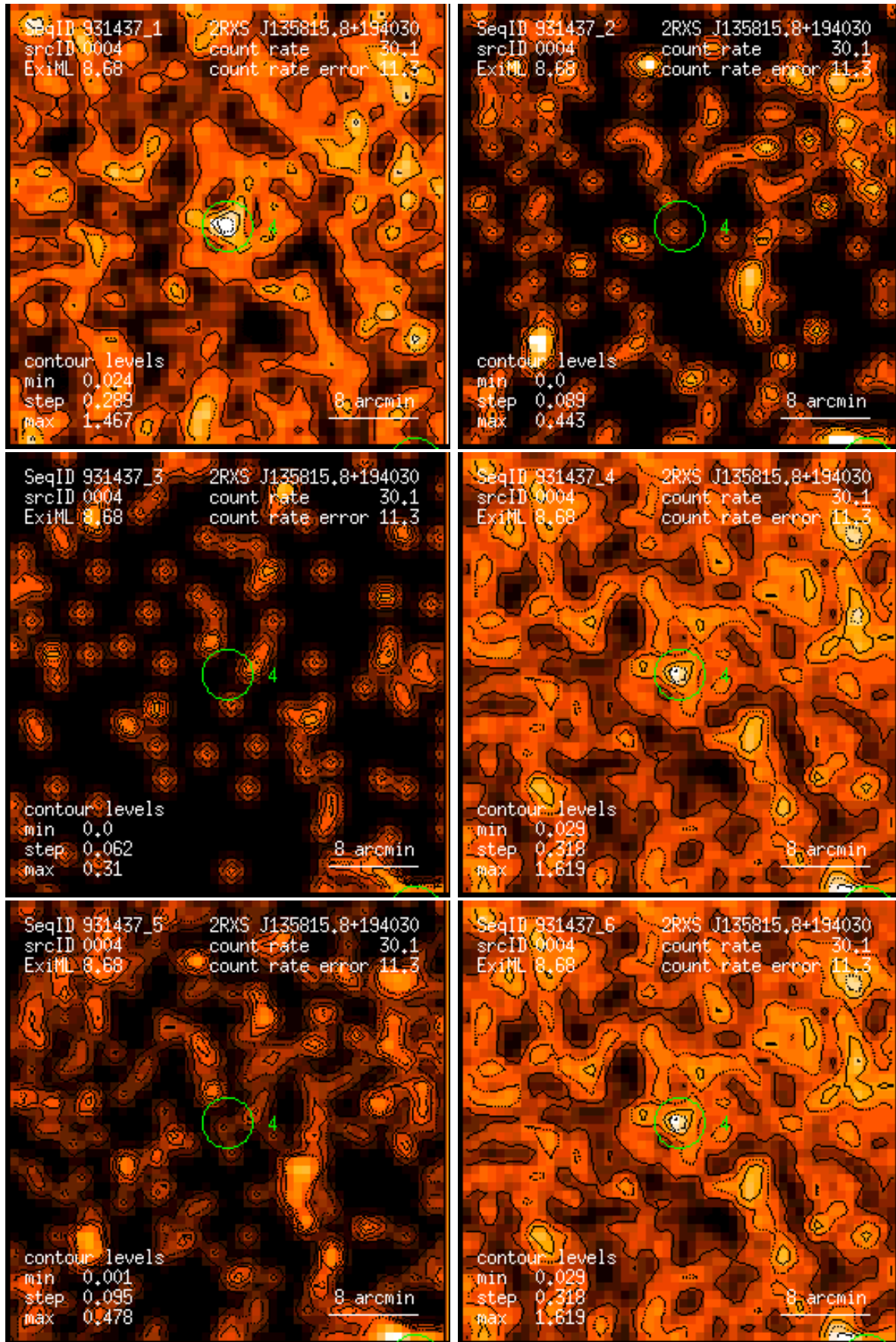
Figure 4: RASS 931437: detection 0004: band rate images, Gaussian filter: (1) PSPC channels 11 – 41, (2) 52 – 90, (3) 91 – 201, (4) 11 – 235, (5) 52 – 201, (6) 11 – 201. Broad band rates in counts/ks. Band rate contour levels in counts/ks/arcmin 2 .
