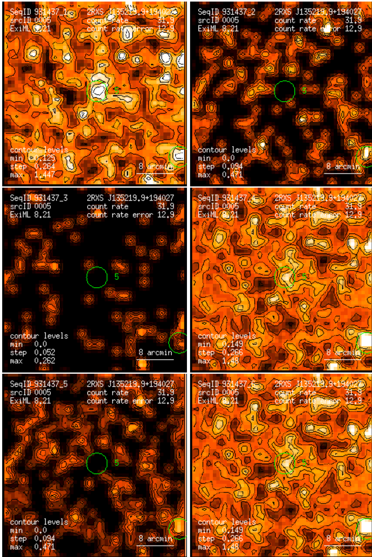
Figure 5: RASS 931437: detection 0005: band rate images, Gaussian filter: (1) PSPC channels 11 – 41, (2) 52 – 90, (3) 91 – 201, (4) 11 – 235, (5) 52 – 201, (6) 11 – 201. Broad band rates in counts/ks. Band rate contour levels in counts/ks/arcmin 2 .
