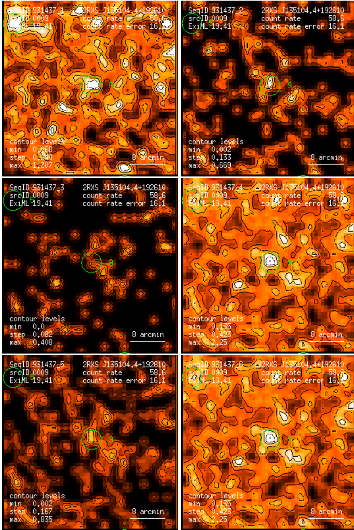
Figure 9: RASS 931437: detection 0009: band rate images, Gaussian filter: (1) PSPC channels 11 – 41, (2) 52 – 90, (3) 91 – 201, (4) 11 – 235, (5) 52 – 201, (6) 11 – 201. Broad band rates in counts/ks. Band rate contour levels in counts/ks/arcmin 2 .
