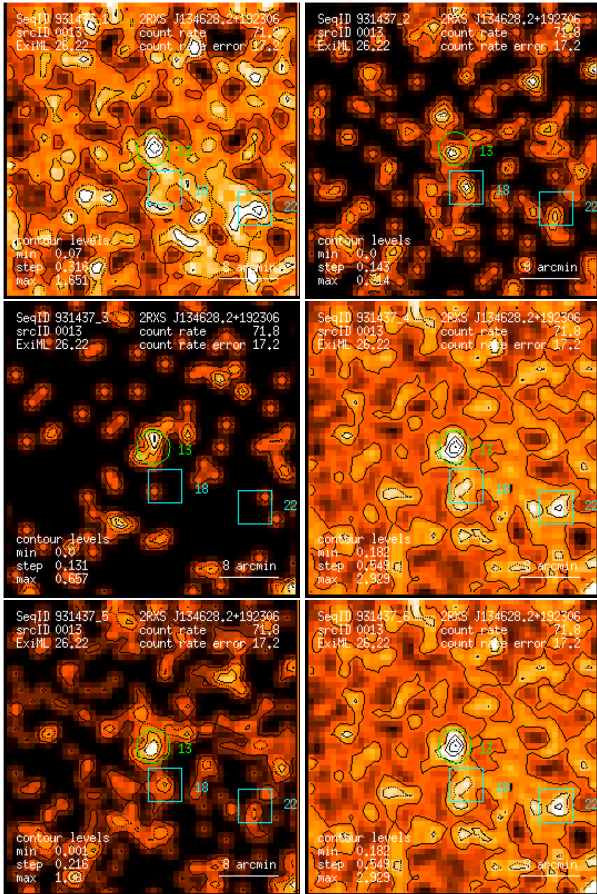
Figure 13: RASS 931437: detection 0013: band rate images, Gaussian filter: (1) PSPC channels 11 – 41, (2) 52 – 90, (3) 91 – 201, (4) 11 – 235, (5) 52 – 201, (6) 11 – 201. Broad band rates in counts/ks. Band rate contour levels in counts/ks/arcmin 2 .
