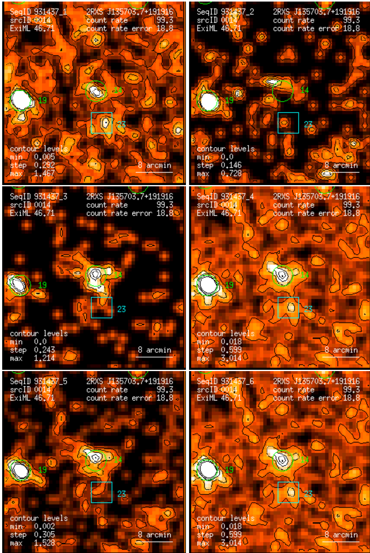
Figure 14: RASS 931437: detection 0014: band rate images, Gaussian filter: (1) PSPC channels 11 – 41, (2) 52 – 90, (3) 91 – 201, (4) 11 – 235, (5) 52 – 201, (6) 11 – 201. Broad band rates in counts/ks. Band rate contour levels in counts/ks/arcmin 2 .
