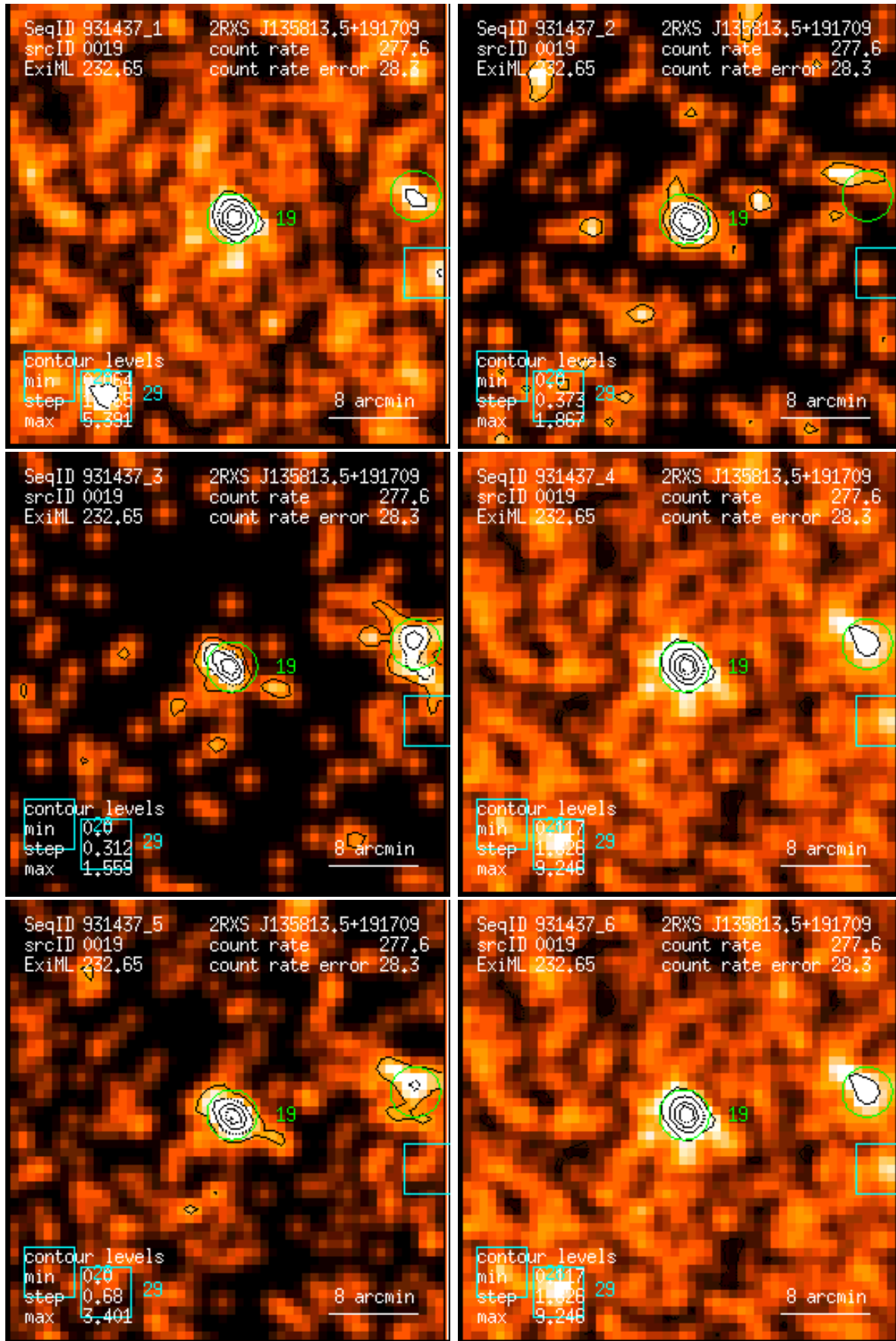
Figure 19: RASS 931437: detection 0019: band rate images, Gaussian filter: (1) PSPC channels 11 – 41, (2) 52 – 90, (3) 91 – 201, (4) 11 – 235, (5) 52 – 201, (6) 11 – 201. Broad band rates in counts/ks. Band rate contour levels in counts/ks/arcmin 2 .
