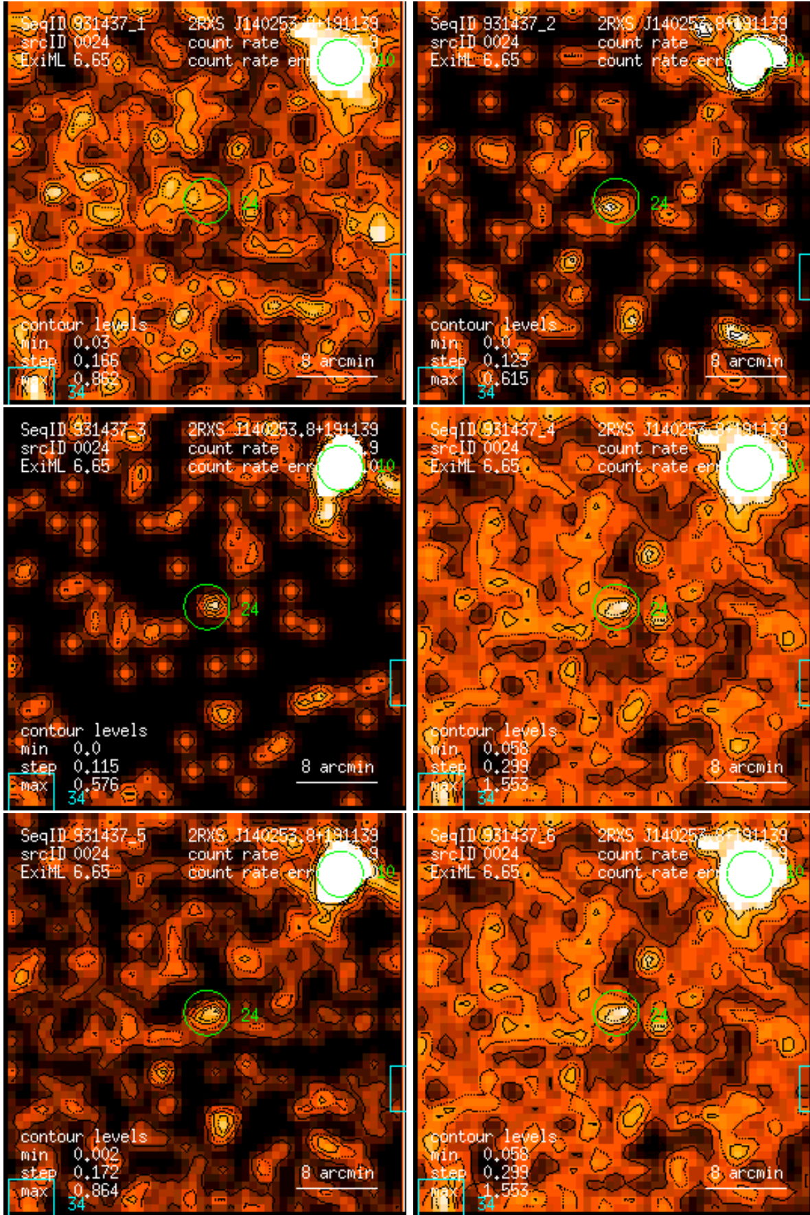
Figure 24: RASS 931437: detection 0024: band rate images, Gaussian filter: (1) PSPC channels 11 – 41, (2) 52 – 90, (3) 91 – 201, (4) 11 – 235, (5) 52 – 201, (6) 11 – 201. Broad band rates in counts/ks. Band rate contour levels in counts/ks/arcmin 2 .
