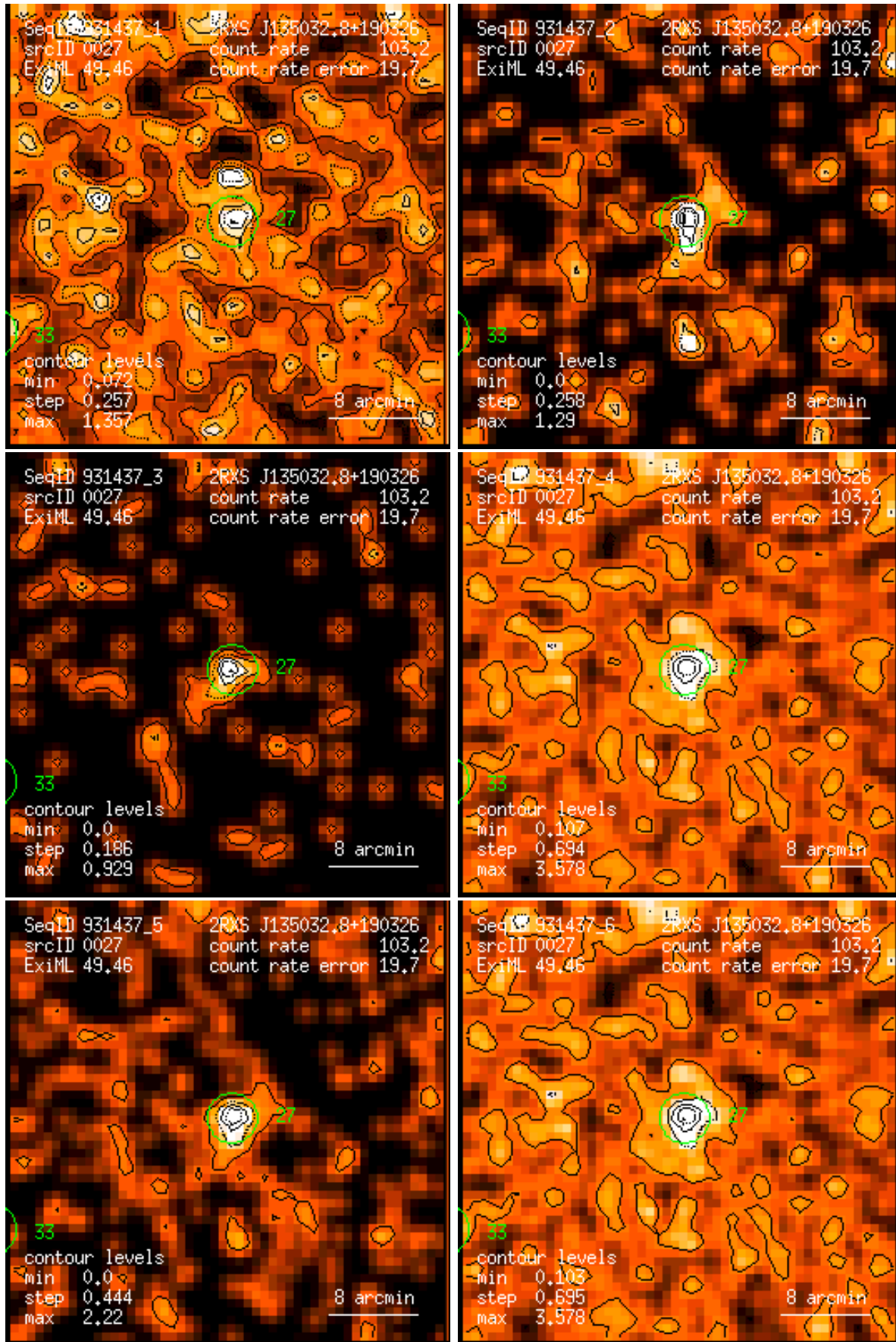
Figure 27: RASS 931437: detection 0027: band rate images, Gaussian filter: (1) PSPC channels 11 – 41, (2) 52 – 90, (3) 91 – 201, (4) 11 – 235, (5) 52 – 201, (6) 11 – 201. Broad band rates in counts/ks. Band rate contour levels in counts/ks/arcmin 2 .
