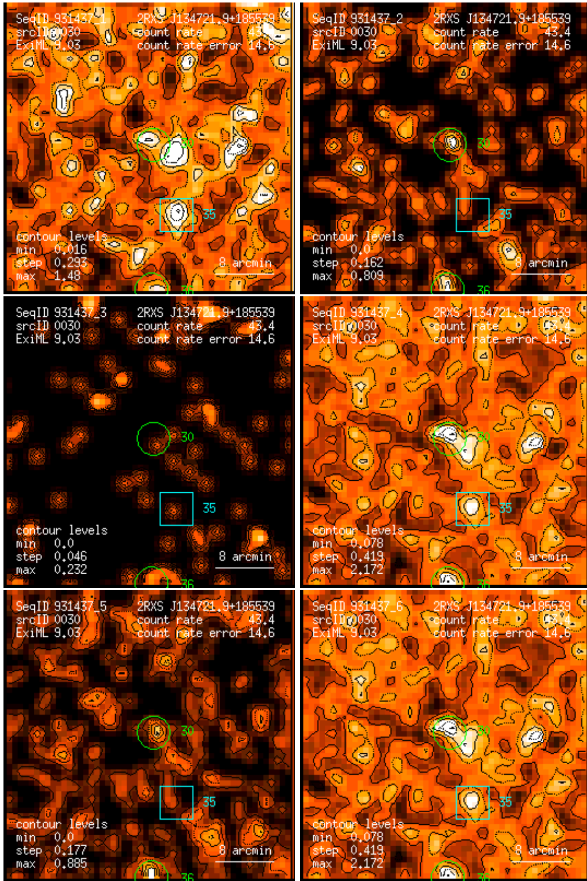
Figure 30: RASS 931437: detection 0030: band rate images, Gaussian filter: (1) PSPC channels 11 – 41, (2) 52 – 90, (3) 91 – 201, (4) 11 – 235, (5) 52 – 201, (6) 11 – 201. Broad band rates in counts/ks. Band rate contour levels in counts/ks/arcmin 2 .
